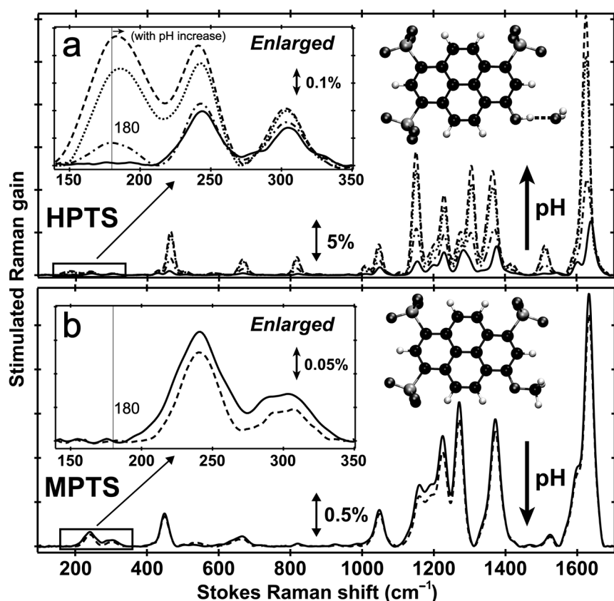
Fig. 1 Ground-state FSRS of 40 mM HPTS and 20 mM MPTS in \text{H}_2\text{O} . (a) HPTS in \text{H}_2\text{O} at pH=4.5 (solid), 7 (dash-dotted), 9 (dotted), and 12 (dashed line) from \sim 100 – 1700\text{ cm}^{-1} . The enlarged low-frequency region between 140 – 350\text{ cm}^{-1} is shown in the insert (left). (b) MPTS in \text{H}_2\text{O} at pH=4.5 (solid) and 12 (dashed line). The enlarged low-frequency region is shown. Molecular structures of HPTS (H-bonded to one nearby water molecule) and MPTS are depicted in the insert (right). Carbon, oxygen, and hydrogen atoms are depicted in black, dark gray, and white spheres, respectively. The Raman gain magnitude is indicated by the double-headed line. The largely featureless aqueous solvent blank spectrum has been subtracted. Notably, we only use this high sample concentration to enhance ground-state vibrational peaks particularly in the low-frequency region.
