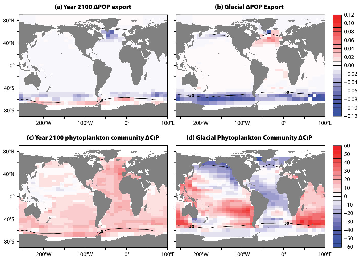
FIGURE 3. Experiment-minus-control changes under global warming and glacial conditions. The change in particulate organic phosphorus ( \Delta\text{POP} ) export (mole-P \text{m}^{-2} \text{ yr}^{-1} ) for (a) year 2100, and (b) glacial. Phytoplankton community \Delta\text{C:P} (molar ratio) for (c) year 2100 and (d) glacial. The black line indicates mean annual sea ice coverage of 50% (e.g., 100% coverage for half a year) predicted by the model under prevailing climate conditions.
