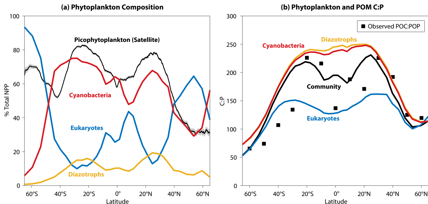
FIGURE 2. Annual mean properties in the control model for the top 100 m of the water column. (a) Zonally averaged, net primary production (NPP)-weighted phytoplankton community composition. The three phytoplankton functional types (PFTs) represented in the model are eukaryotes (blue), cyanobacteria (red), and diazotrophs (yellow). The black line is the remotely sensed contribution of picophytoplankton (0.5–2 \mu m) to total carbon-based biomass (Kostadinov et al., 2016). (b) Zonally averaged C:P uptake ratios for each PFT (colored lines) and the NPP-weighted community C:P (black line). The community C:P would be reflected in the C:P ratio of organic particles. Black squares are based on data from C:P from Martiny et al. (2013).
