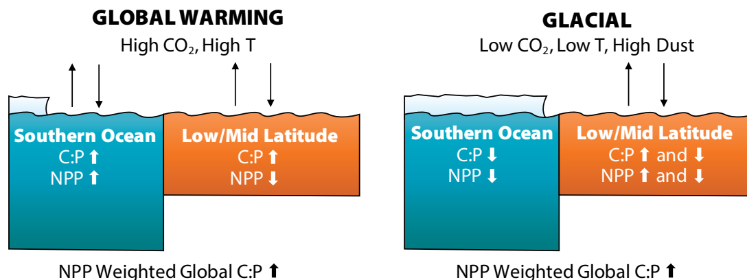
FIGURE 4. A schematic diagram illustrating the differences in two model conditions. In the global warming scenario (left), both C:P and net primary production (NPP) increase in the Southern Ocean as sea ice retreats and nutrient utilization increases. In the low/mid latitudes, C:P rises as nutrient availability decreases and temperatures rise. In the glacial scenario (right), both NPP and C:P in the Southern Ocean decrease as sea ice expands and nutrient utilization decreases. In the low/mid latitudes, the responses of C:P and NPP vary regionally.
