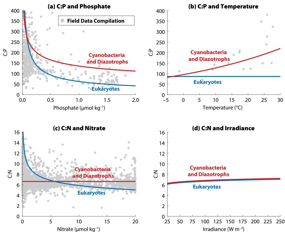
FIGURE 1. C:P and C:N ratios of three phytoplankton groups as functions of four environmental drivers with sensitivities from the meta-analysis of Tanioka and Matsumoto (2020). In each panel, only one driver is changed while others are kept constant at reference values. The gray dots are C:P and C:N data of bulk particulate organic matter from the field. (a) and (c) from Galbraith and Martiny (2015) and (b) from Yvon-Durocher et al. (2015)
