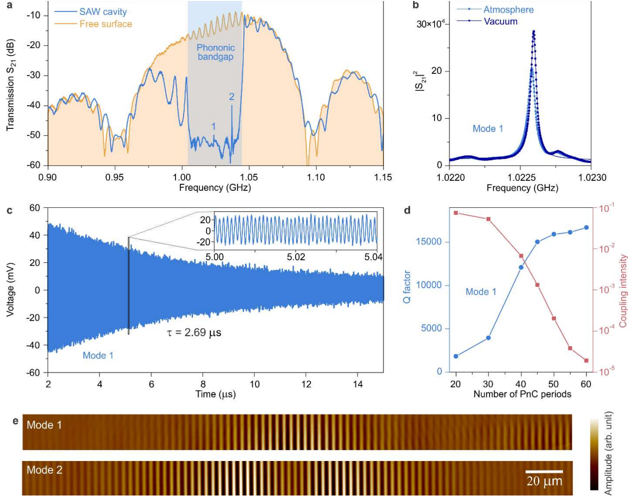
Figure 3 | Measurements of high-Q SAW resonator on lithium niobate. a , Transmission measurements of a SAW resonator and an unperturbed free surface using a pair of IDT. Two high-Q modes, labeled 1 and 2, are observed in the bandgap of the PnC. b , Fine scans of transmission measurements for the Mode 1 in atmosphere and vacuum. The measured data (dots) are fitted to Lorentzian peaks (lines). c , Resonator ring down measurement of Mode 1 showing a lifetime of 2.69 \mu s. Inset: the voltage oscillation around 5 \mu s. d , Measurements of Q factors and coupling intensities of Mode 1 of resonators with different numbers of PnC periods. Coupling intensity is measured as the peak height in transmission. e , Measurements of SAW mode profiles using transmission-mode microwave impedance microscopy, showing mode profiles as a fundamental mode for Mode 1, and a second-order mode for Mode 2. This is the top view of the device.
