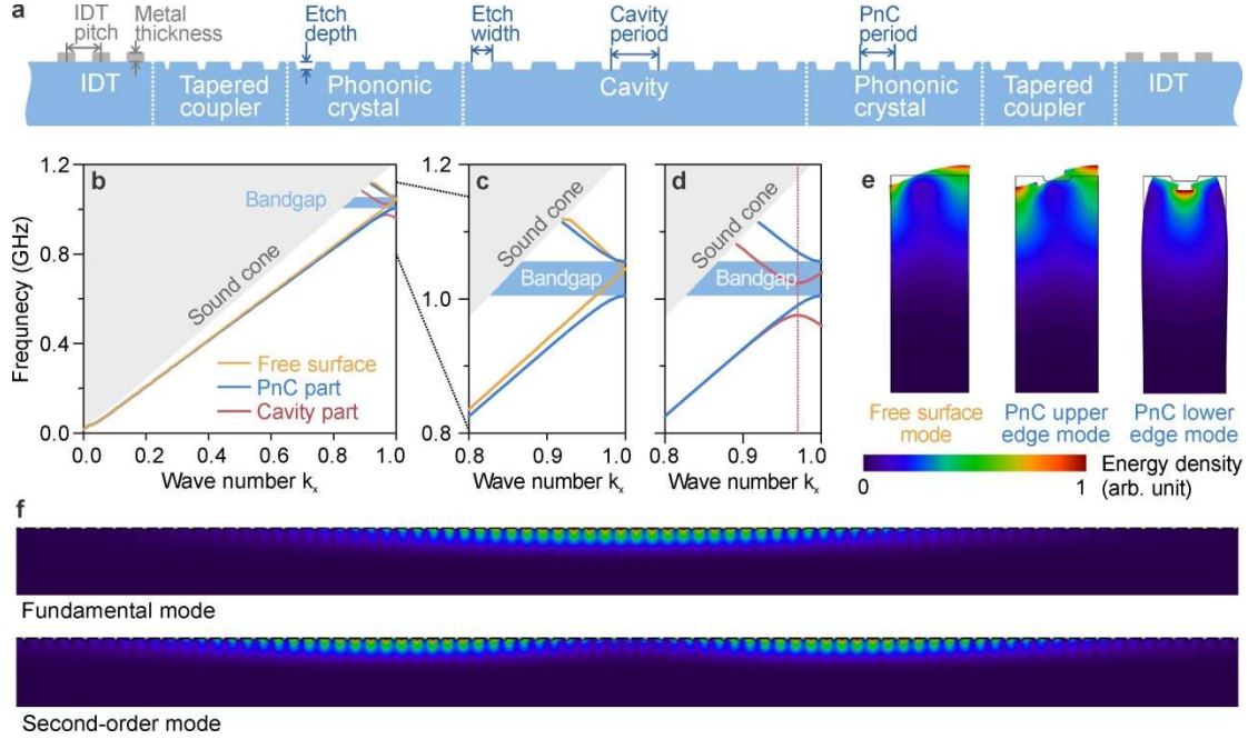
Figure 2 | Phononic band structure engineering of surface acoustic wave (SAW) on lithium niobate. a , Schematic of the SAW resonator and its design parameters. b-d , Phononic band structures for SAW on unperturbed free surface, surface phononic crystal (PnC) part, and cavity part. The wave number k_x is normalized to the \pi phase of PnC. The vertical red dash line indicates the \pi of the cavity part, which is of a greater period. The design parameters are: etch width 0.653 \mu\text{m} , etch depth 115 nm, period for PnC part 1.92 \mu\text{m} , and period for cavity part 1.98 \mu\text{m} . e , SAW modes of free surface and PnC with \pi phase of the unit cells. f , Mode profiles of the fundamental and second-order mode of the SAW resonator. The color scale indicates the total energy density of electromagnetic, kinetic, and elastic energy densities.
