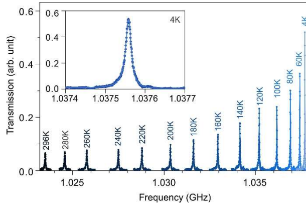
Figure 4 | Low-temperature measurements of SAW resonators. Transmission ( |S_{21}|^2 ) of the fundamental mode measured during the sample cooling down by continuous flow liquid helium, and the temperature is monitored by a thermal coupler on the sample mount. Inset: A fine scan of the fundamental mode at the stabilized temperature of 4K.
