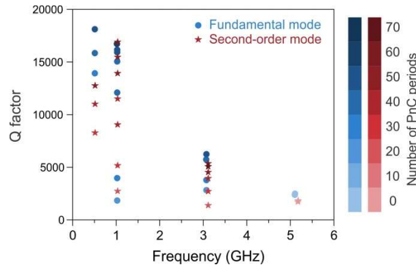
Figure 5 | Q factors on resonant frequencies of SAW resonators in atmosphere. The fundamental modes and the second-order modes are marked in blue circles and red stars, respectively. The color scale represents the number of PnC periods fabricated to confine the SAW modes.
