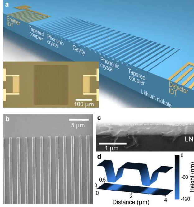
Figure 1 | Surface acoustic wave resonator on lithium niobate. a , Illustration of band structure engineered surface acoustic resonator on lithium niobate. Inset: optical microscope image of a fabricated device. The dark region at the center is the etched grooves, and the bright regions on the sides are metal IDTs. b , Scanning electron microscope image of the cavity part on lithium niobate. c , Cross-section showing the etched grooves at the cavity part. A platinum layer is deposited to protect the surface of lithium niobate (LN) from damage during focused ion beam milling. d , Surface profile of the SAW resonator scanned by atomic force microscopy.
