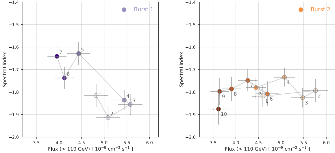
Figure 3. Photon index vs. flux of the VERITAS detections of Mrk 421 over 5 minute intervals shown separately for bursts 1 (left) and 2 (right). The colors represent the chronological progression of the bursts, with lighter colors corresponding to earlier times. The indices are obtained by a fit with an exponential cutoff power law ( E_{\text{cut}} ), where E_{\text{cut}} is fixed to the global value of 4 TeV. The data behind this figure and Figure 2 are available in FITS format.
