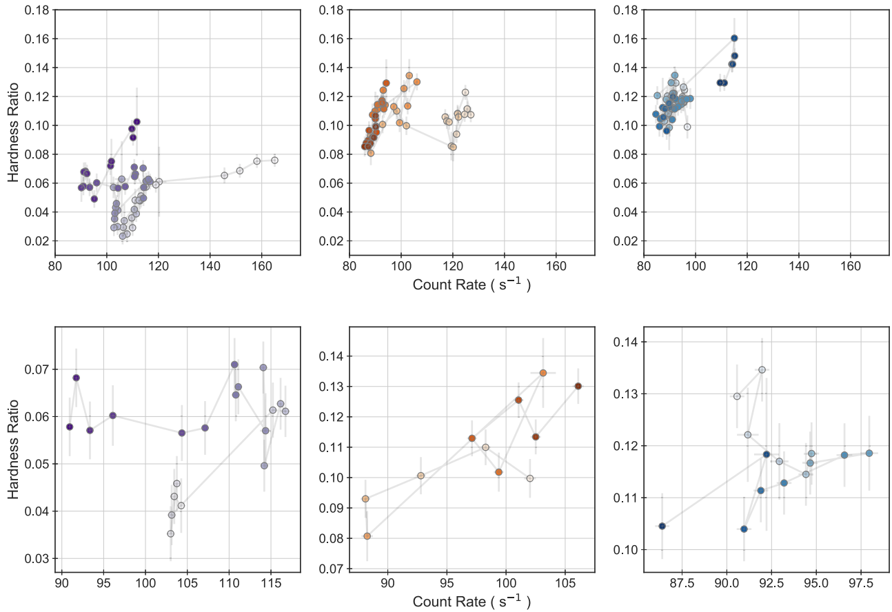
Figure 13. Top panels: hardness ratio (between 5–15 and 3–5 keV) vs. count rate of the RXTE observations of Mrk 421 over the three decline epochs indicated by the arrows in Figure 6 (not strictly simultaneous with VHE data within the epoch). Left: epoch 4; middle: epoch 5; right: epoch 6. The color shading of the data points represents the chronological progression of the bursts, with lighter colors corresponding to earlier times. Bottom panels: zoom-in on hardness ratio vs. count rate of the RXTE observations of Mrk 421 corresponding to the colored bands in Figure 6 (not strictly simultaneous with VHE data within the epoch). Left: epoch 4 zoom-in; middle: epoch 5 zoom-in; right: epoch 6 zoom-in. The color shading of the data points represents the chronological progression of the bursts, with lighter colors corresponding to earlier times.
