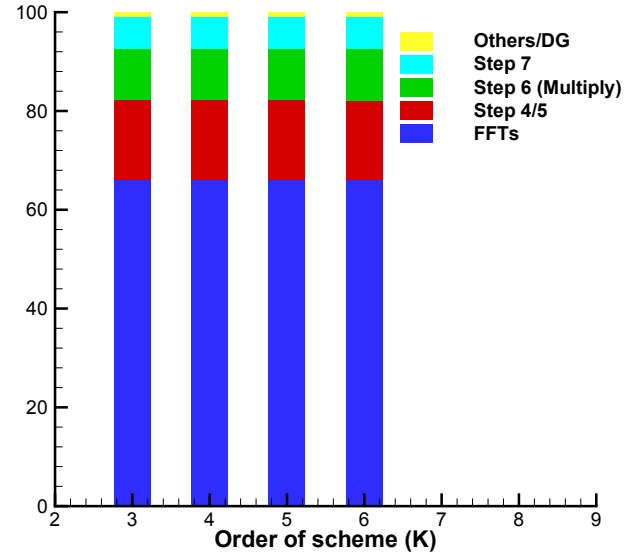
(b) N_e = 72 , N^3 = 32^3
