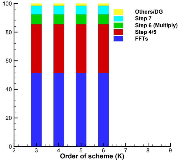
(a) N_e = 72 , N^3 = 20^3
