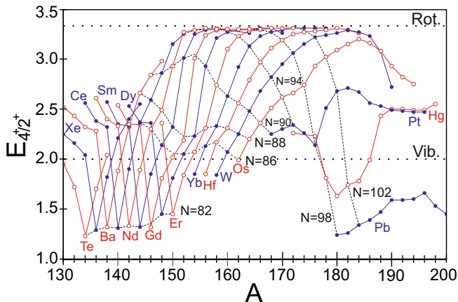
FIG. 1: Ratio of the excitation energies of the lowest 4^+ to 2^+ level in even-even nuclei as a function of mass A , which illustrates the evolution of collectivity in the rare-earth region. This work discusses trends at high spin in Er, Yb, Hf, and W nuclei with 88 \leq N \leq 103 .
