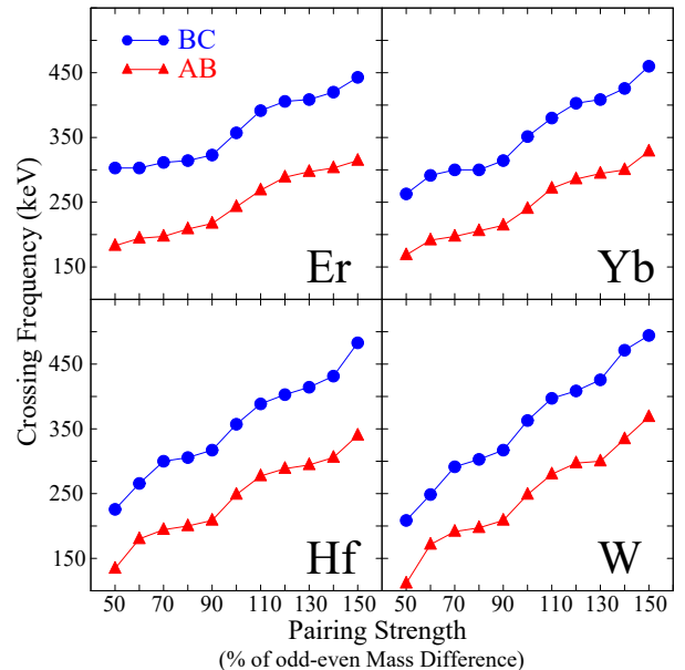
FIG. 7: Calculated AB and BC crossing frequencies plotted as a function of the percentage of the odd-even mass difference for Er, Yb, Hf, and W N = 94 isotones. Deformation values are taken from [39]. Note that the AB and BC trajectories are roughly parallel to one another and that the slopes do not change significantly with proton number.
