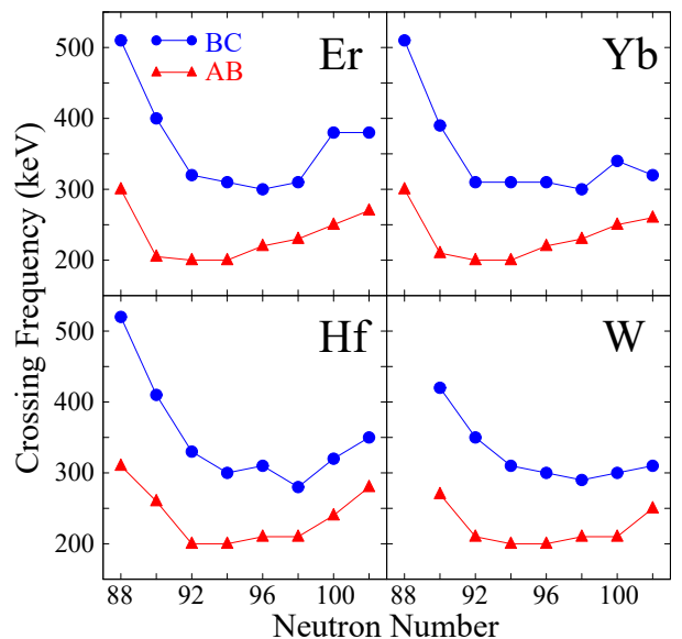
FIG. 3: Theoretical AB and BC crossing frequencies in even-even nuclei, extracted from cranking calculations using a Woods-Saxon potential with pairing. The deformation values were taken from [39] with the pairing strength corresponding to 80% of the odd-even mass difference.
