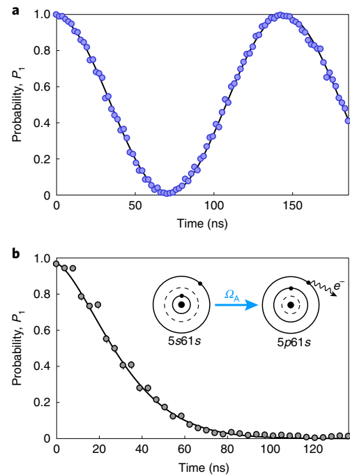
Fig. 2 | Rabi oscillations and auto-ionization. a , Array-averaged probability P_1 of detecting an atom after a resonant Rydberg pulse and subsequent auto-ionization as a function of Rydberg pulse time, showing high-contrast Rabi oscillations with frequency \Omega_R = 2\pi \times 6.80(2) MHz. The auto-ionization pulse time is fixed to 5\ \mu\text{s} . b , P_1 as a function of auto-ionization pulse time at a fixed Rydberg pulse time of 70 ns corresponding to a \pi -pulse (followed by a second \pi -pulse). The solid line is a fit to a Gaussian, phenomenologically chosen to capture the finite switch-on time of the auto-ionization beam (see Supplementary Information). Inset: illustration of the auto-ionization process. In both a and b , data are uncorrected and averaged over ~40-100 experimental cycles per time step and over an array of ~14 atoms. Error bars indicate a 1\sigma binomial confidence interval.
