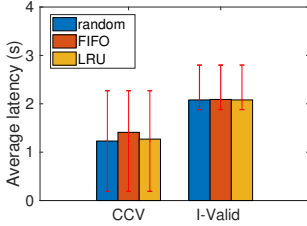
Fig. 5. Validation latency with cache replacement strategies
