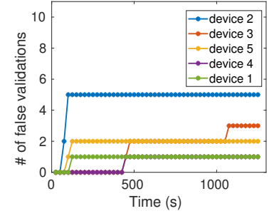
Fig. 8. Number of false validations
