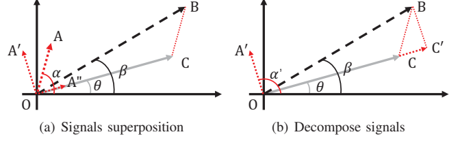
Fig. 1. Relationships between \beta and \theta
