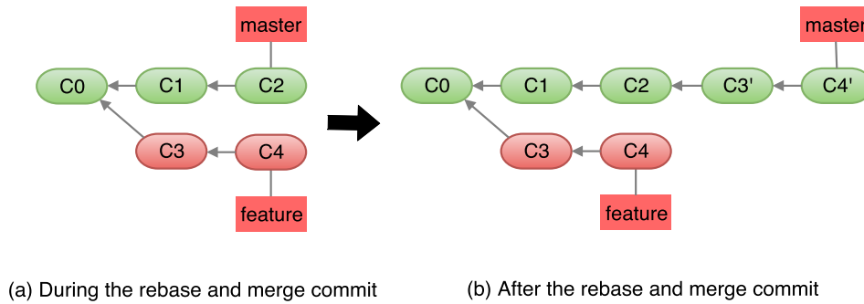
Fig. 6. Repository state for rebase-and-merge operations.
