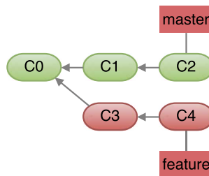
Fig. 1. A Git repo with two branches, master and feature .
