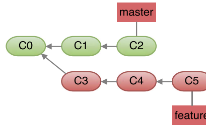
Fig. 3. A regular commit on the feature branch.
