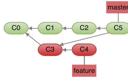
Fig. 7. Incorrect history merge attack.
