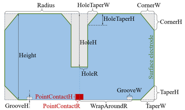
Fig. 28 Cross section along z -axis of an inverted coaxial point-contact HPGe detector, and parameters describing its dimensions. To shorten the names, width is represented as a single capital case “W”, height “H”, and radius “R”
