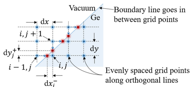
Fig. 20 Variable distances between grid points in case of a boundary line goes in between
