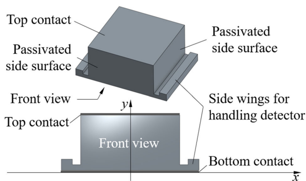
Fig. 33 Configuration of a realistic planar detector that has two side wings for the handling of the detector. The top and bottom surfaces are electrical contacts, the side surfaces are passivated
