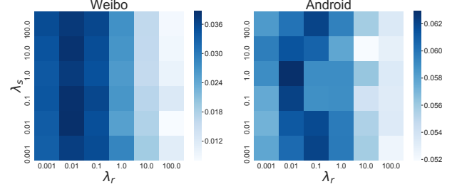
Figure 5: MAP@10 on varying \lambda_s, \lambda_r over Android and Weibo. Performance is more sensitive to variations in \lambda_r than \lambda_s .
