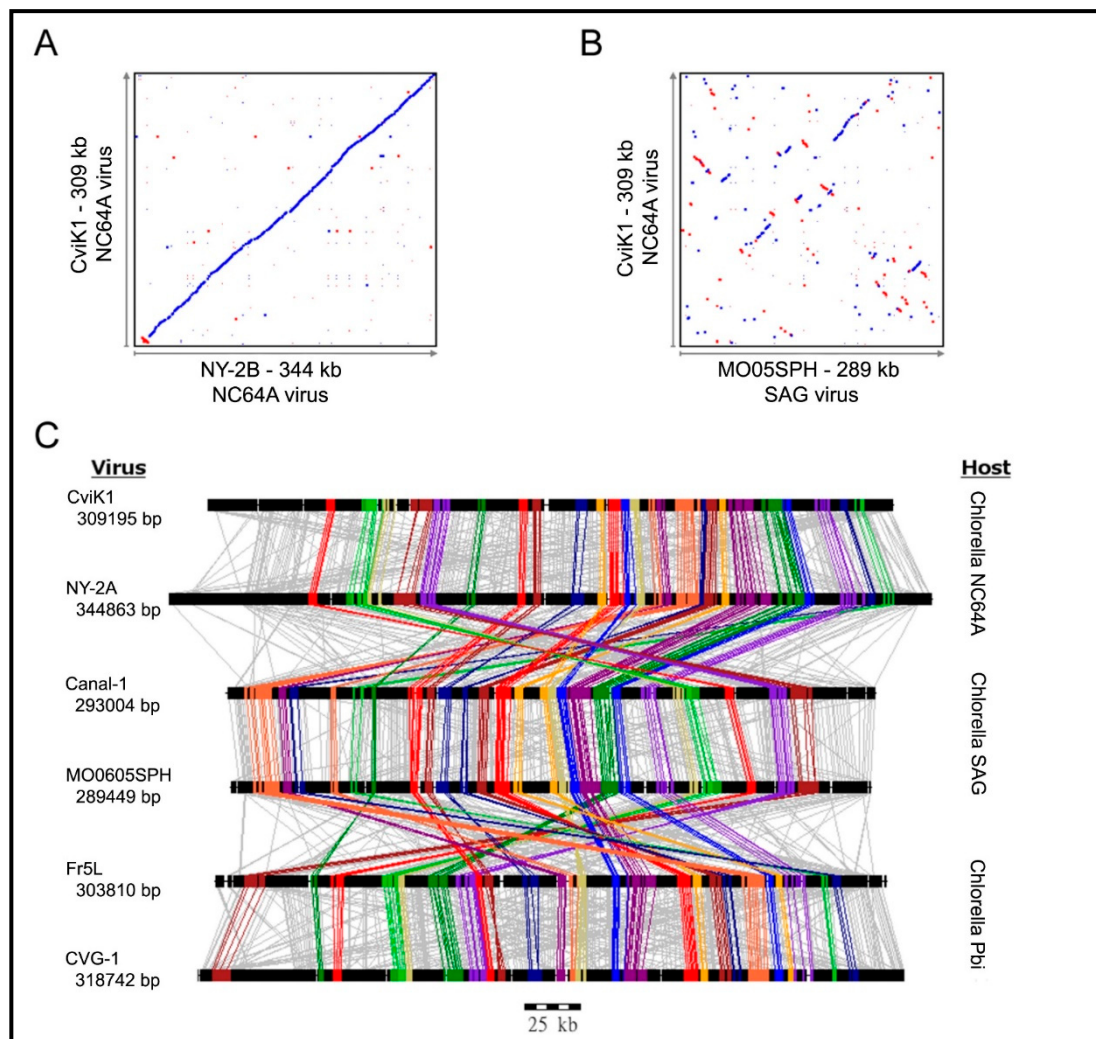
Figure 6. Gene dot-blots and gene alignments across chlorovirus host types. Dot-blot alignments of two chlorovirus genomes infecting the same ( A ) or different ( B ) hosts (blue indicates common genomic orientation, red indicates opposite genomic orientation). Each dot represents a protein match (ortholog) between the two viruses (BLASTp expect value > 1 \times 10^{-5} ). ( C ) Schematic representation of six chlorovirus genomes from three different hosts. Each genome is depicted as a black line with genic regions represented by black boxes. Lines connect genes from the same family of homologous proteins (for clarity purpose, the six bigger families were removed from the figure). The colored set of genes and lines represents the Gene Gangs referred to in the text. While viruses that infect the same host demonstrate good conservation of synteny ( A ), synteny is poorly conserved across the virus types ( B ). Despite generally poor syntenic conservation, gene-centric alignments suggest that some conserved collinear blocks exist ( C ). Figure taken from Seitzer et al. [74] and published with permission.
