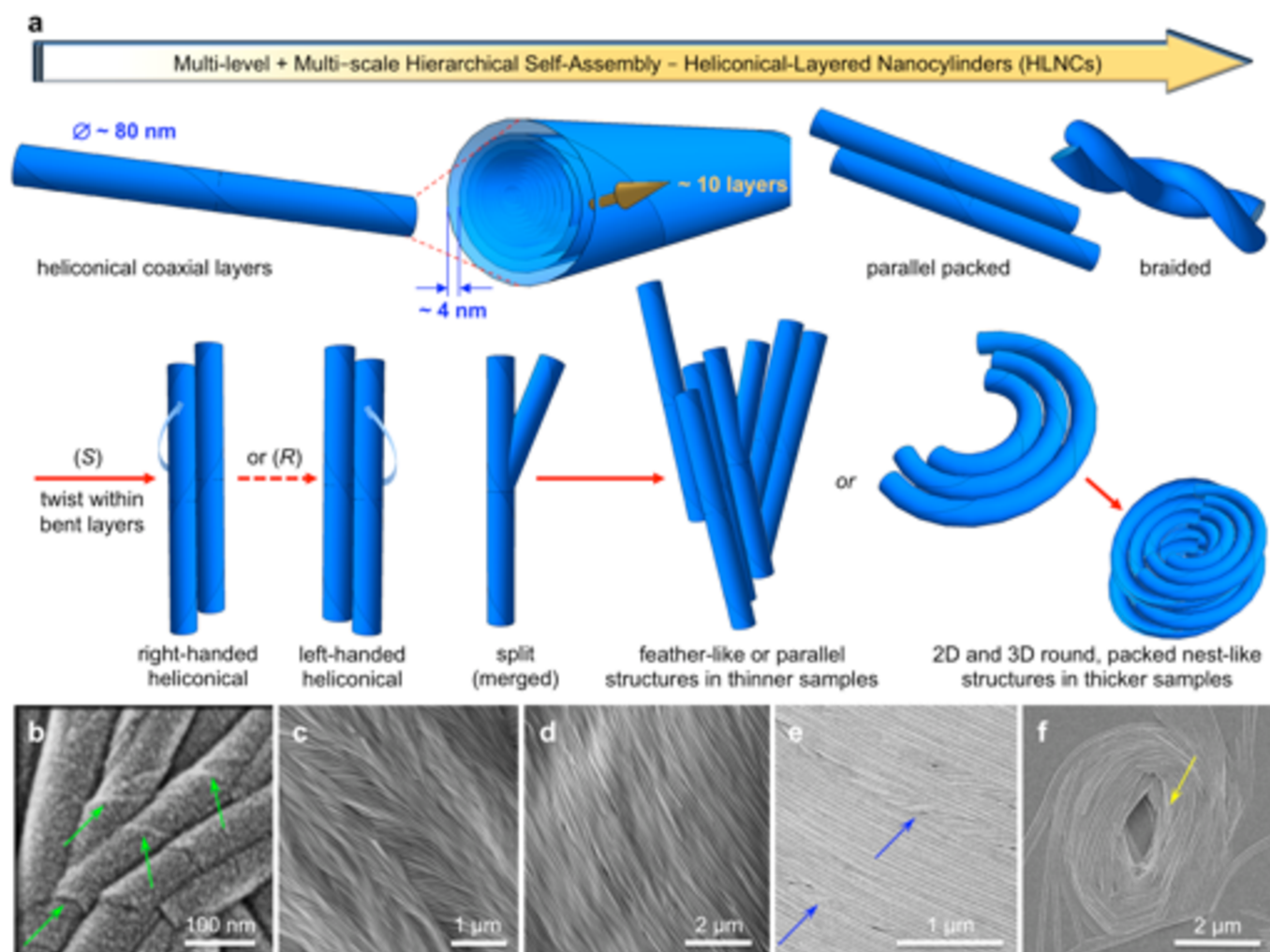
Fig. 5. (a) Models of packing of p -( R )- 4 and p -( S )- 4 in HLNCs and packing modes found for the HLNCs. (b – f) Representative SEM images for the heliconical layers forming the nanocylinders (green arrows in (b)) and the various packing modes (e.g., braided - blue arrows in (e) and birds nest-like – yellow arrow in (f)) observed by SEM, AFM, and TEM.
