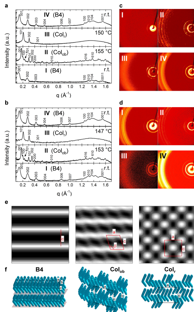
Fig. 3 X-ray diffraction analysis of slow heated and cooled (at 5 °C min -1 ) samples of: (a, c) p -( R )- 4 and (b, d) p -( S )- 4 ; (a, b) azimuthally integrated intensity (a.u.) vs. q (Å -1 ) of (c, d) the corresponding 2D diffraction patterns. Additional synchrotron small angle X-ray diffraction experiments were used to index the B4 (HLNC) and Col ob phases (see ESI, Section 8, Fig. S18 and Table S2). (e) 2-Dimensional electron density maps reconstructed from X-ray data by reverse Fourier transform of the B4 (HLNC), Col ob and Col r phases. Maps show ac plane. The change from black to white indicates increasing electron density. The modulation in-layer along the 'a' direction for the B4 phase is equal a single molecule and therefore not visible. The size of these maps is 15 × 15 nm 2 . The isodensity line is marked to visualize the cross section of the columns. (f) Corresponding molecular models for the B4, Col ob and Col r phase formed by p -( R )- 4 and p -( S )- 4 .
