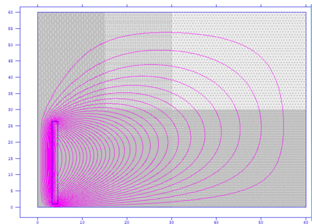
Figure 5: Field lines from the right half of solenoid magnet placed at 1 mm above the superconducting sample.
