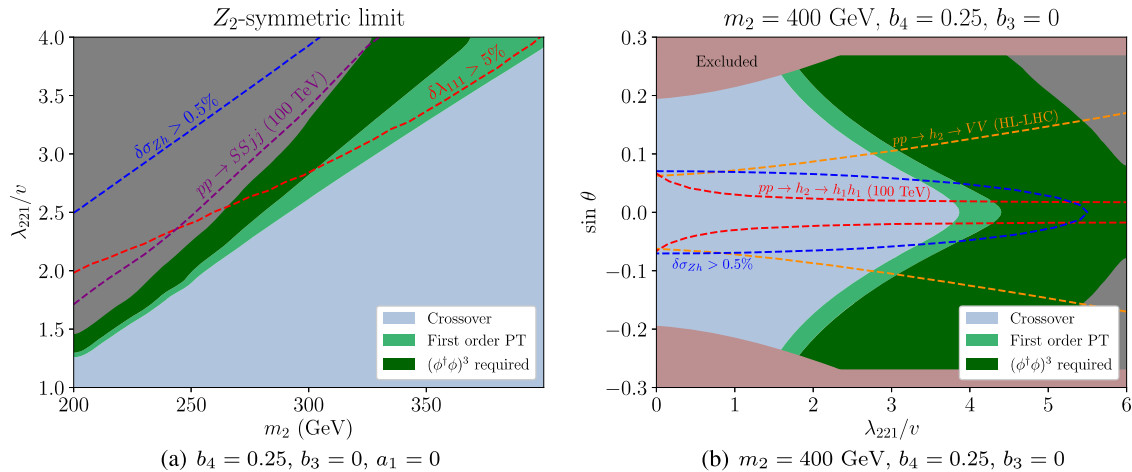
FIG. 6. As in Fig. 3 ( Z_2 ) and the right panel of 4 (non- Z_2 ) but including limits and projections for several collider observables, discussed in the text. The red shaded regions on the right are currently excluded either by the electroweak precision measurements discussed in Ref. [88], or direct searches for the singlet-like scalar in final states involving two gauge bosons [112]. The high luminosity LHC, a future Higgs factory and 100 TeV collider could together probe a significant amount of parameter space consistent with a first-order electroweak phase transition as predicted by our nonperturbative analysis.
