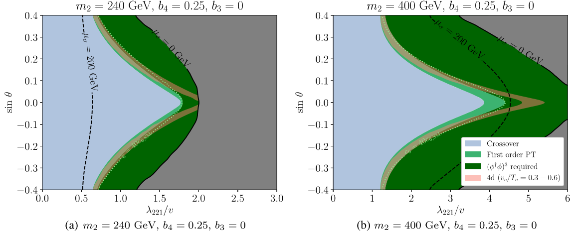
FIG. 4. Parameter space of the xSM predicting a first-order electroweak phase transition for various values of m_2 and \sin \theta with b_3 = 0 , in both the 4-d perturbative and 3-d nonperturbative approaches. The light green regions features a first-order electroweak phase transition as predicted by existing lattice results. The darker shaded region features x < 0 so that the higher dimension operator (\phi^\dagger \phi)^3 must be kept in the dimensionally reduced theory to resolve one-step electroweak transitions. Furthermore, to the right of the dotted green contour, the dimension-6 operator coefficient, c_6 , becomes larger than 40 times the corresponding SM value, c_{6,\text{SM}} , and the neglected (\phi^\dagger \phi)^3 term can already have significant effects. We also show contours indicating the size of the singlet \overline{\text{MS}} mass parameter \mu_\sigma . When \mu_\sigma \lesssim gT \approx 100 GeV, the superheavy singlet approximation becomes compromised. The gray shaded regions correspond to where the singlet mass parameter \mu_\sigma^2 < 0 so that the superheavy dimensional reduction completely breaks down. The parameter space in which 4-d perturbation theory predicts a first-order transition with v_c/T_c = 0.3\text{--}0.6 is shaded orange, and matches up well with the nonperturbative first-order regions especially away from the Z_2 limit, where the couplings required for a first-order EWPT are not as large.
