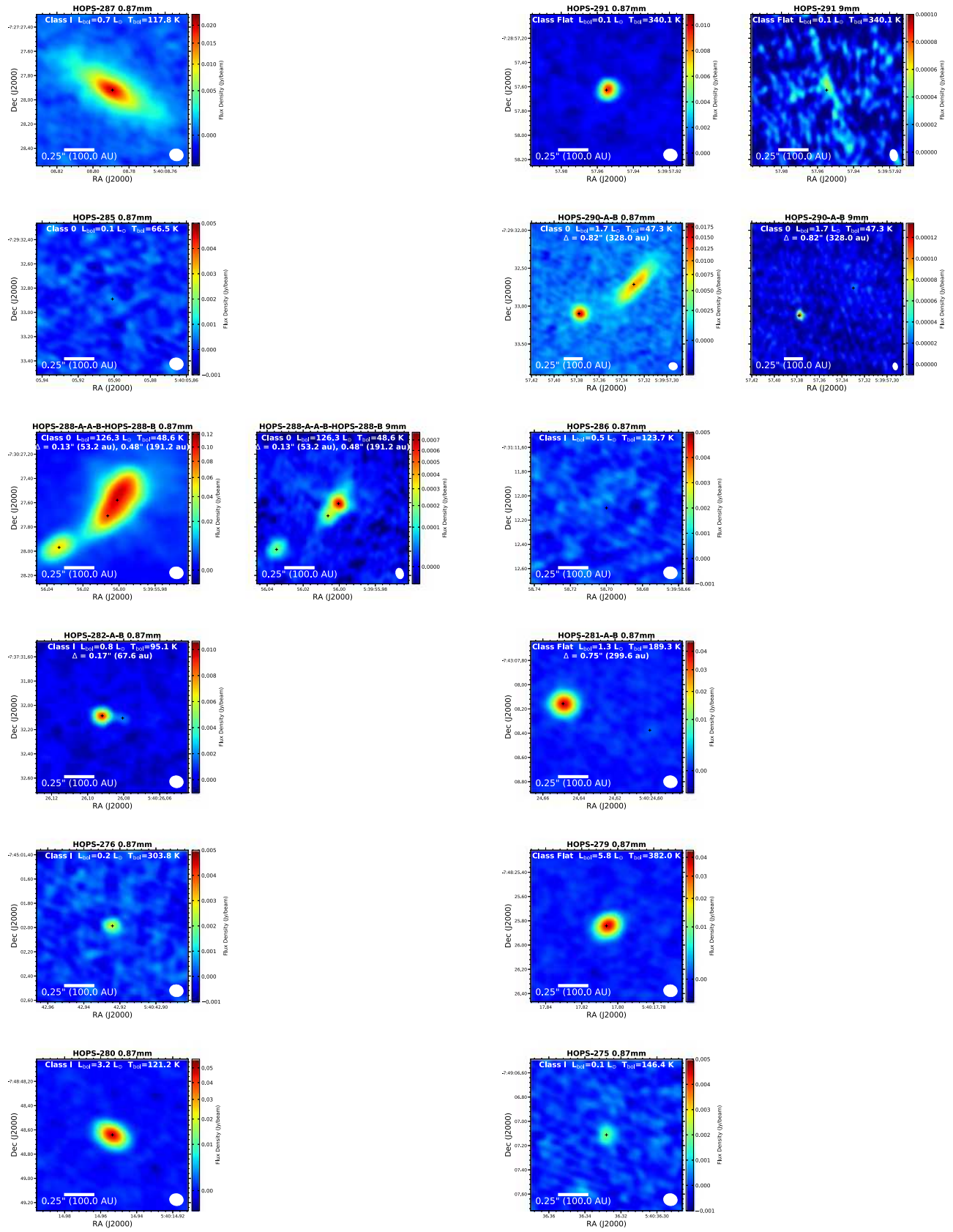
Figure 48. Orion images.
