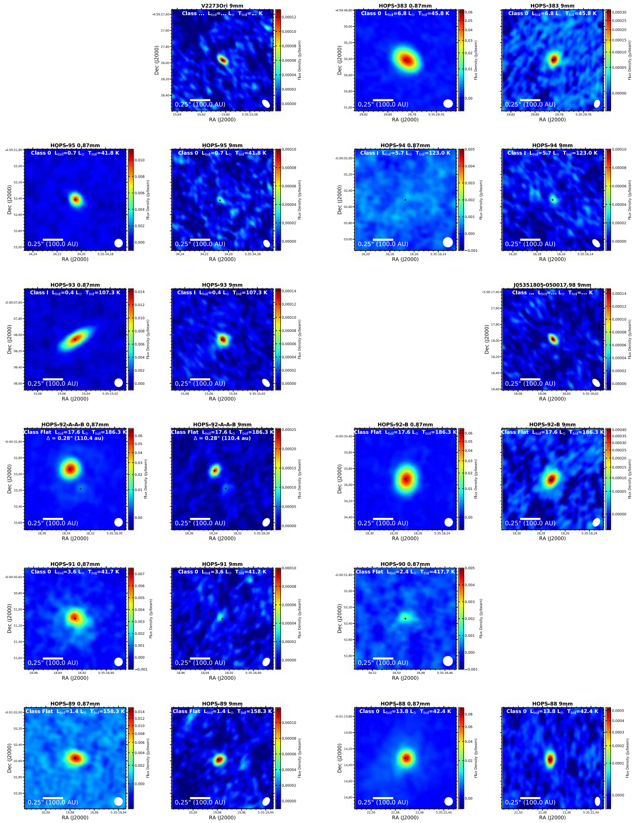
Figure 30. Orion images.
