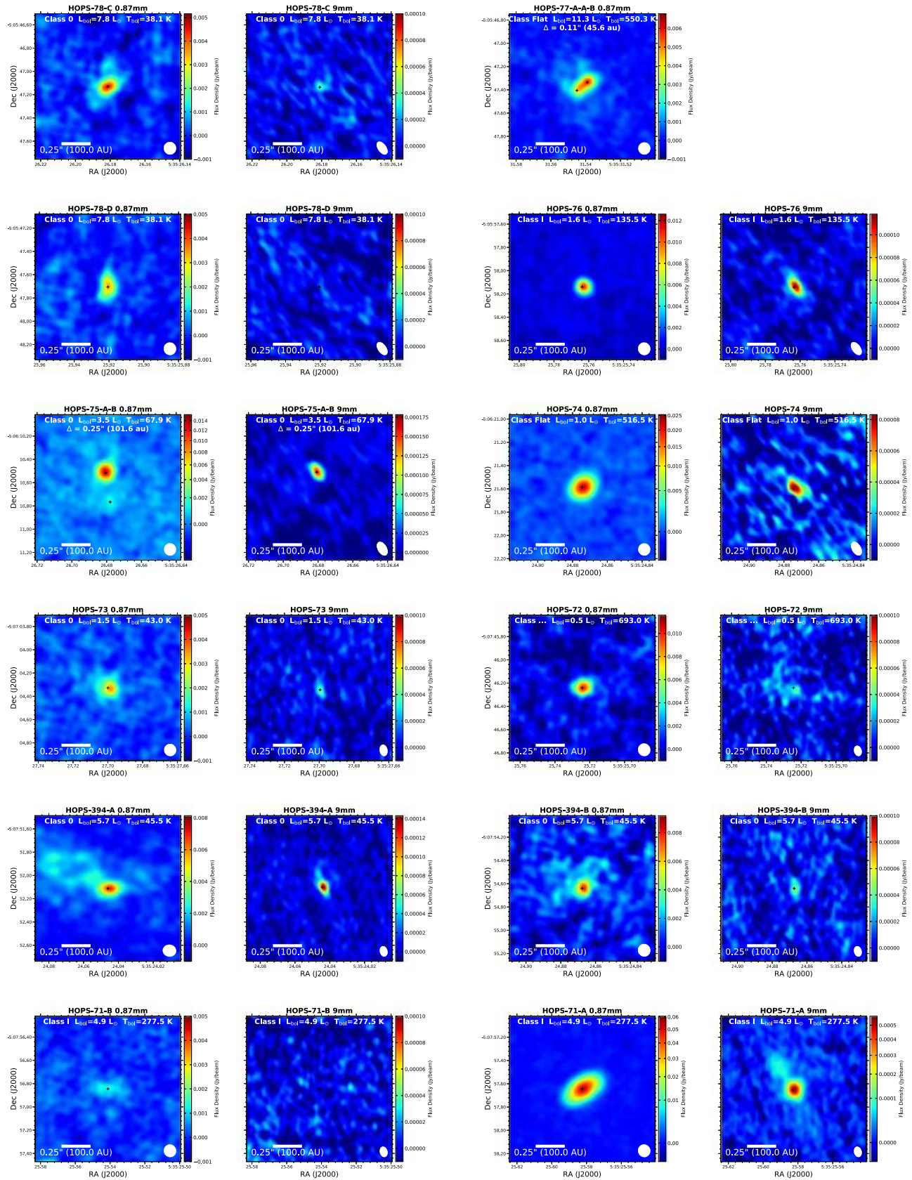
Figure 32. Orion images.
