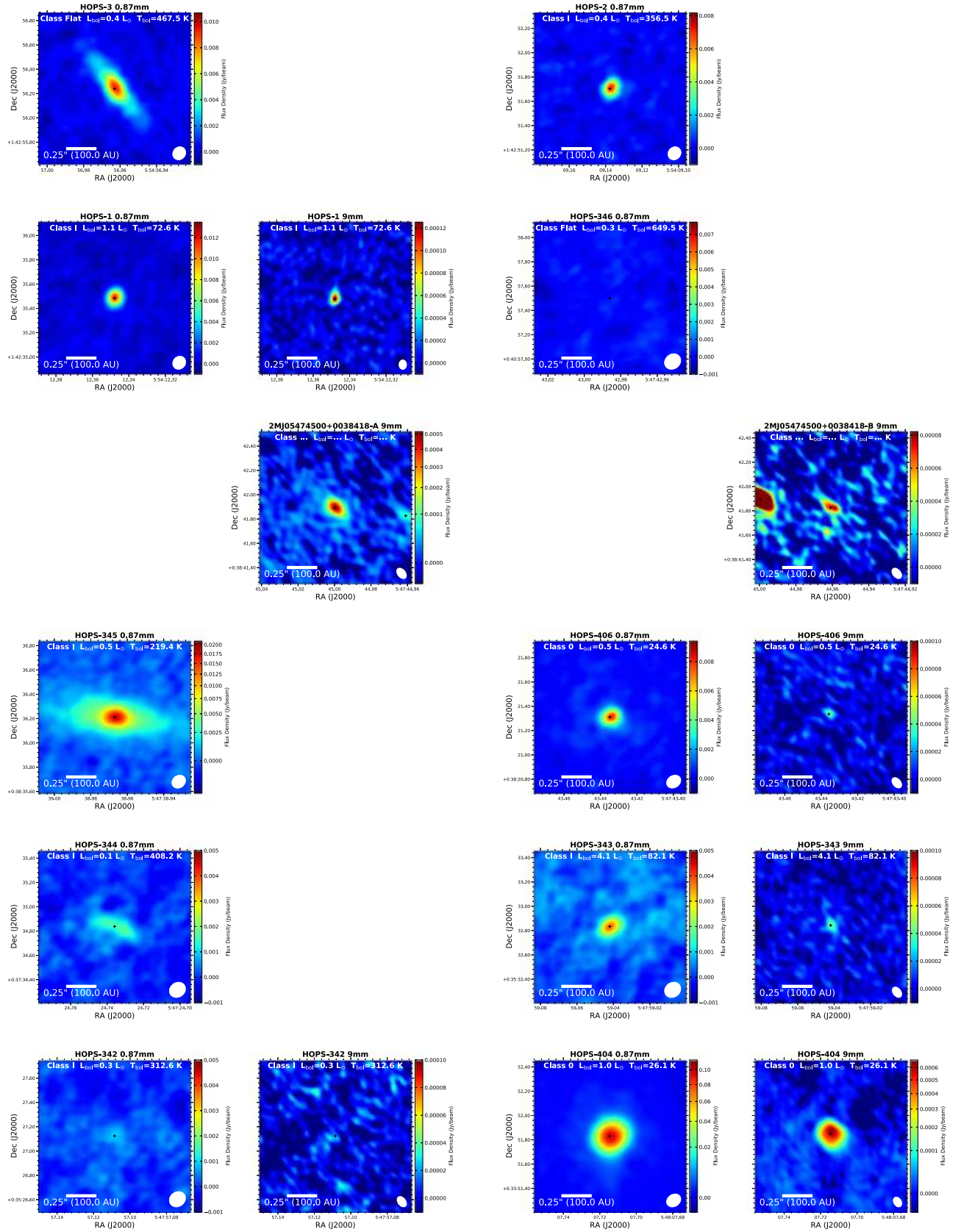
Figure 20. Orion images.
