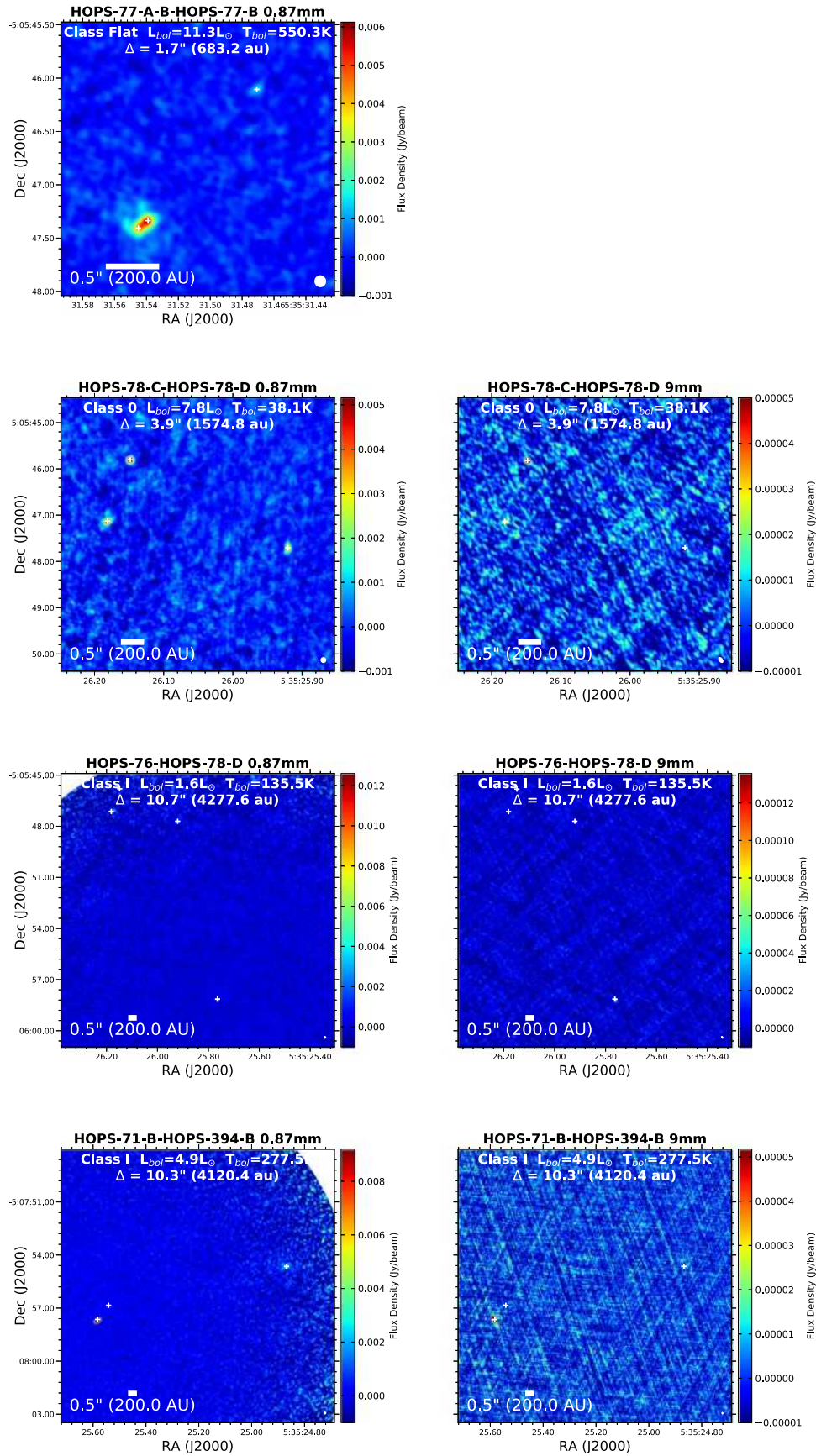
Figure 61. Orion wide multiple images.
