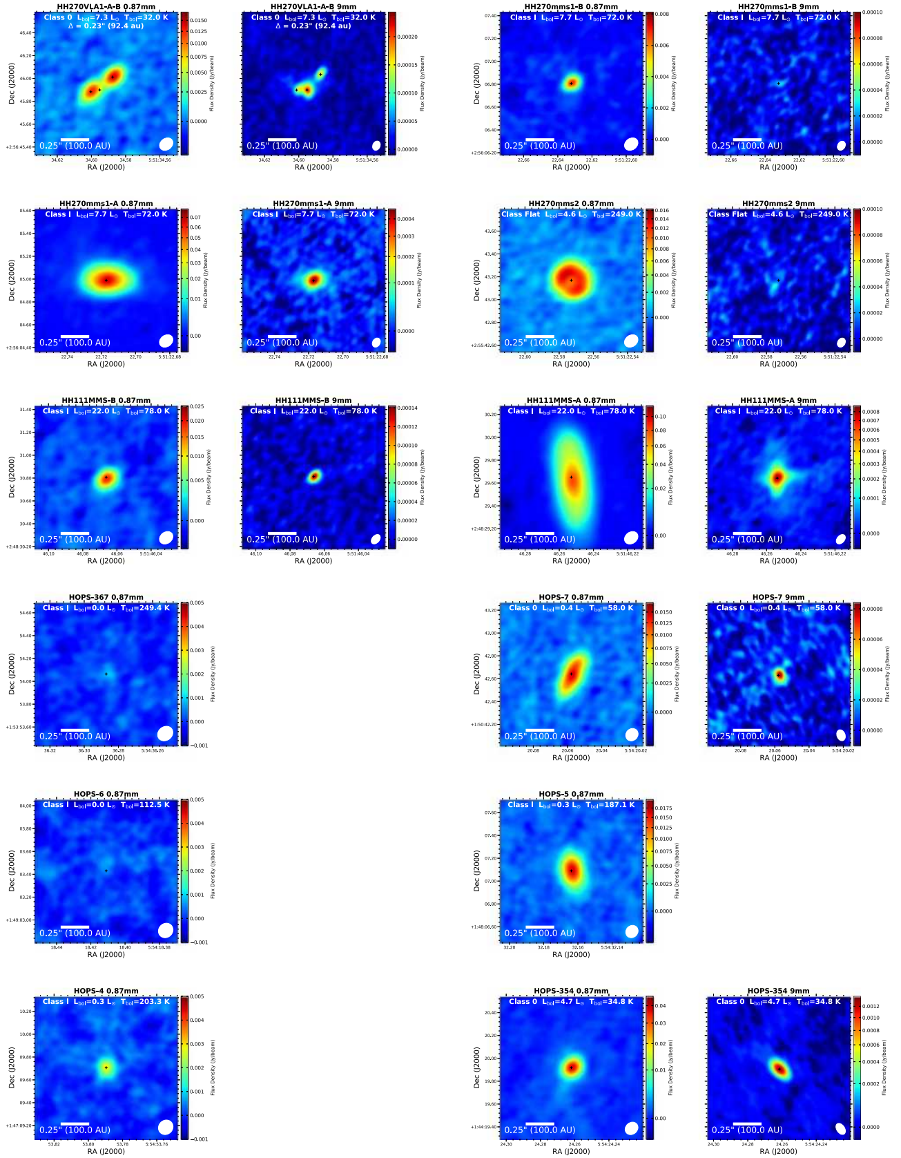
Figure 19. Orion images.
