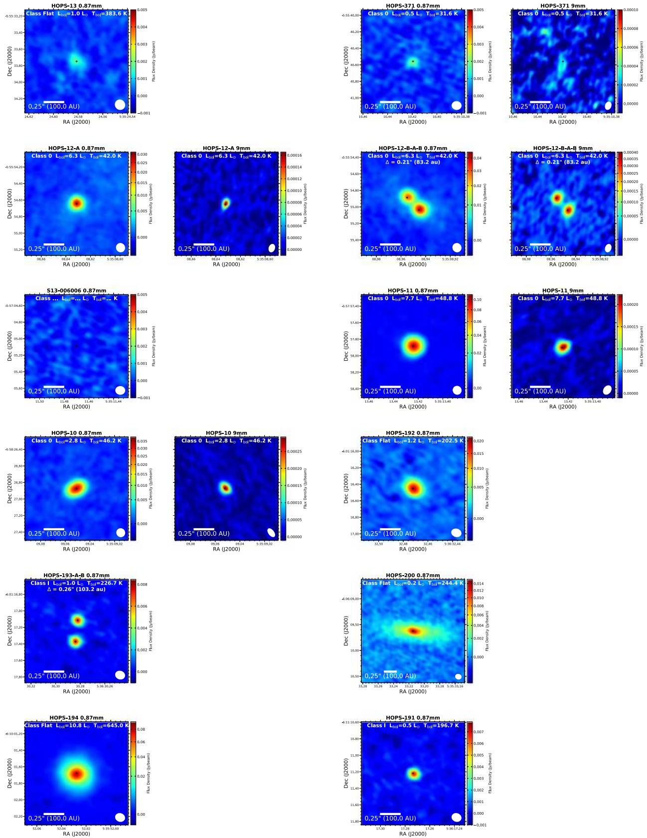
Figure 39. Orion images.
