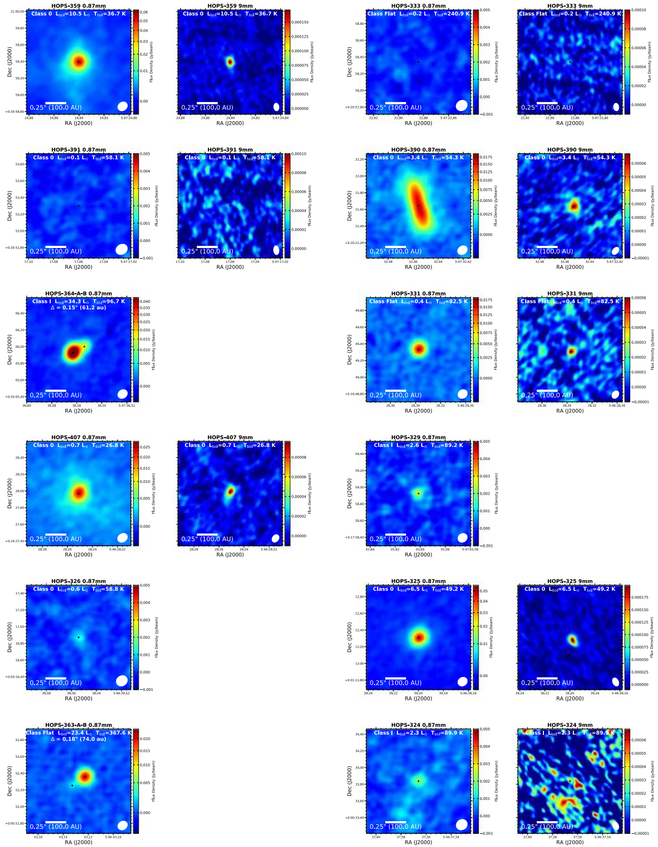
Figure 23. Orion images.
