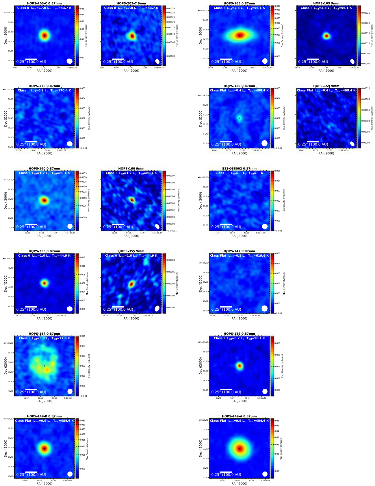
Figure 43. Orion images.
