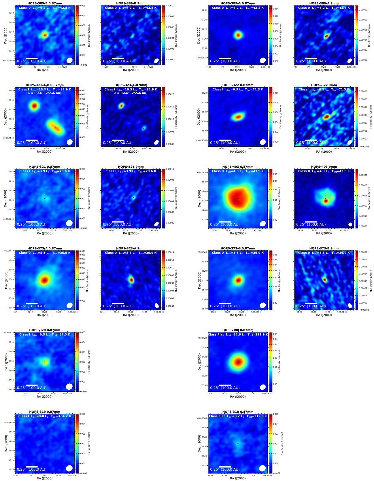
Figure 24. Orion images.
