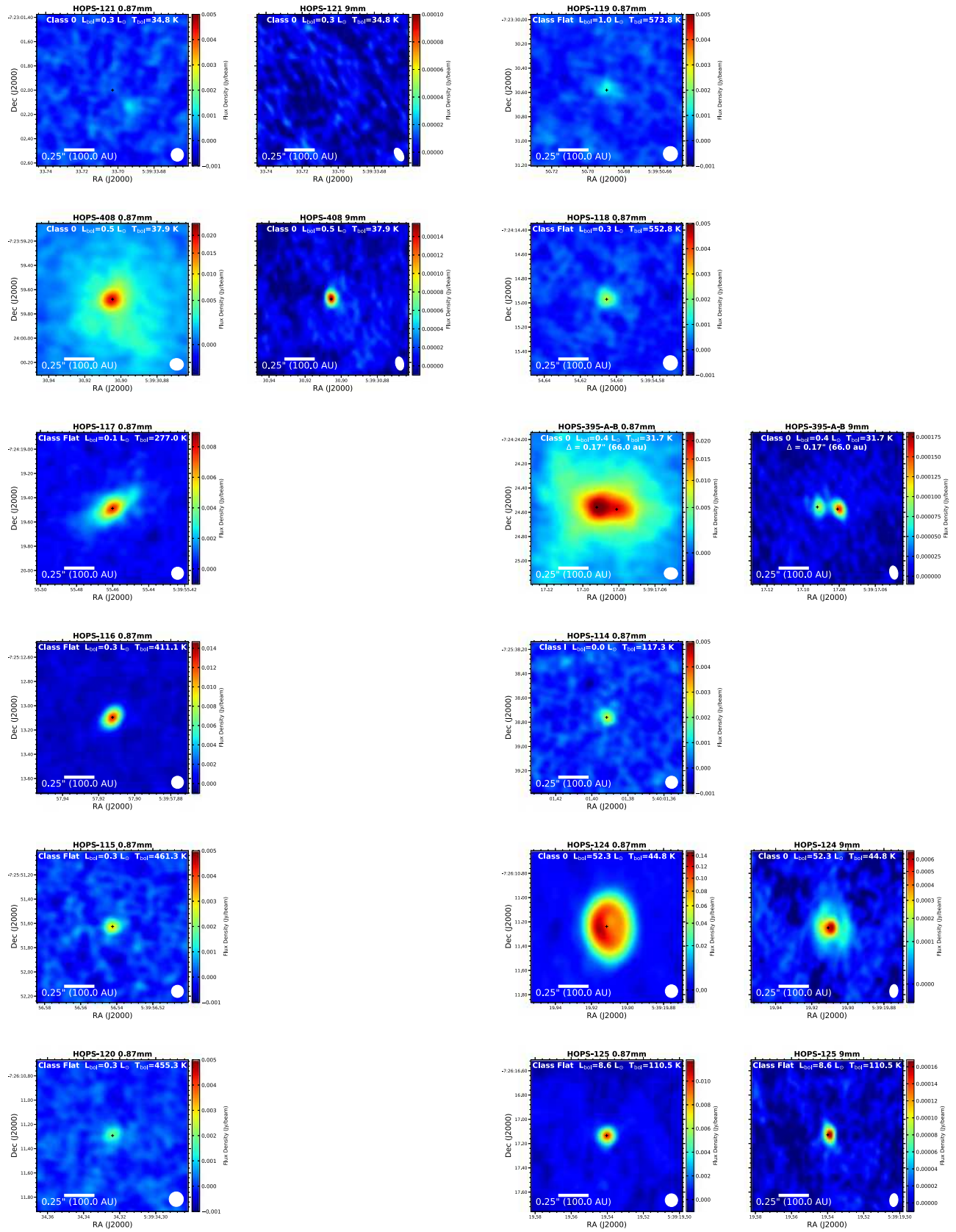
Figure 47. Orion images.
