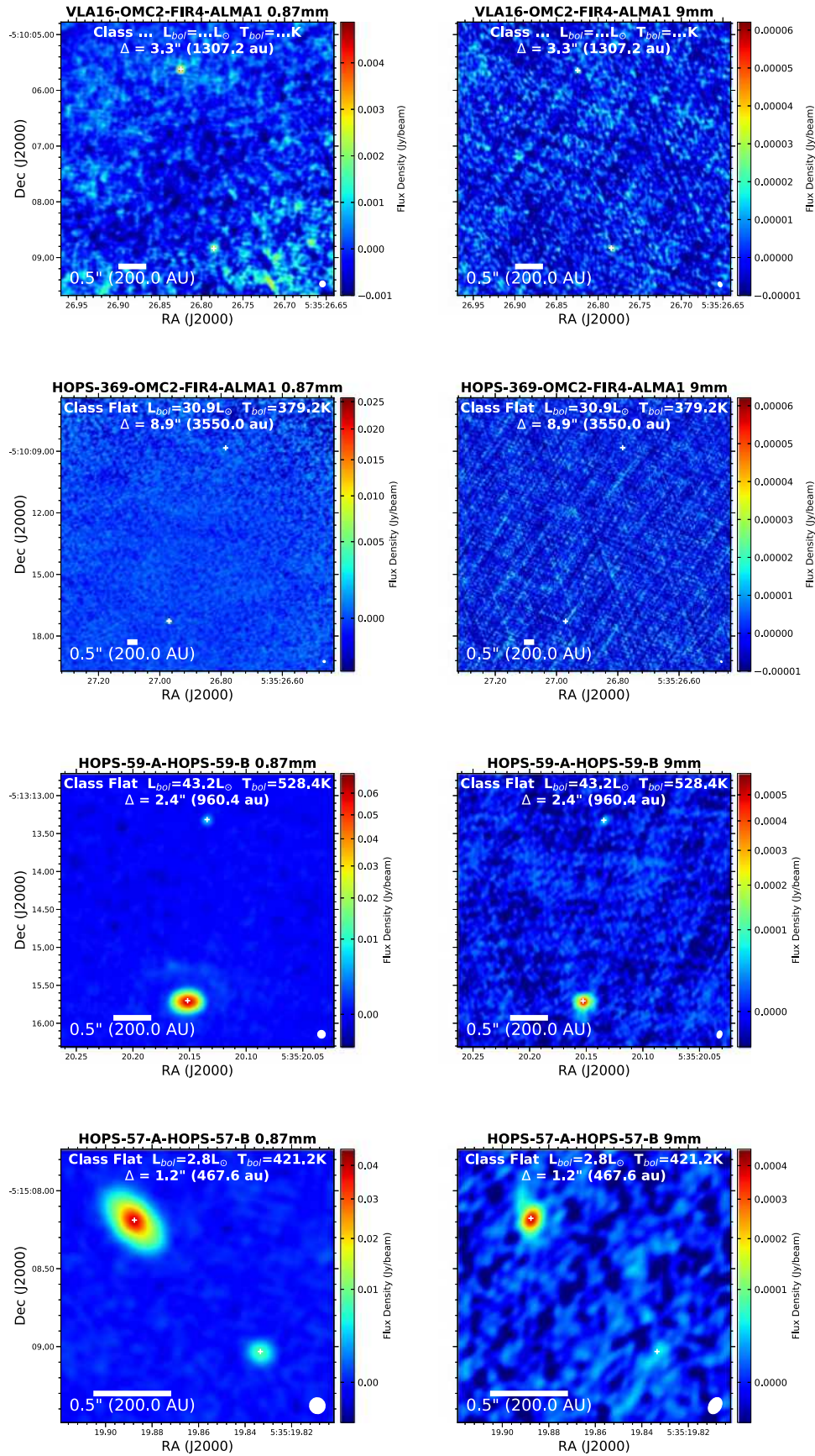
Figure 64. Orion wide multiple images.
