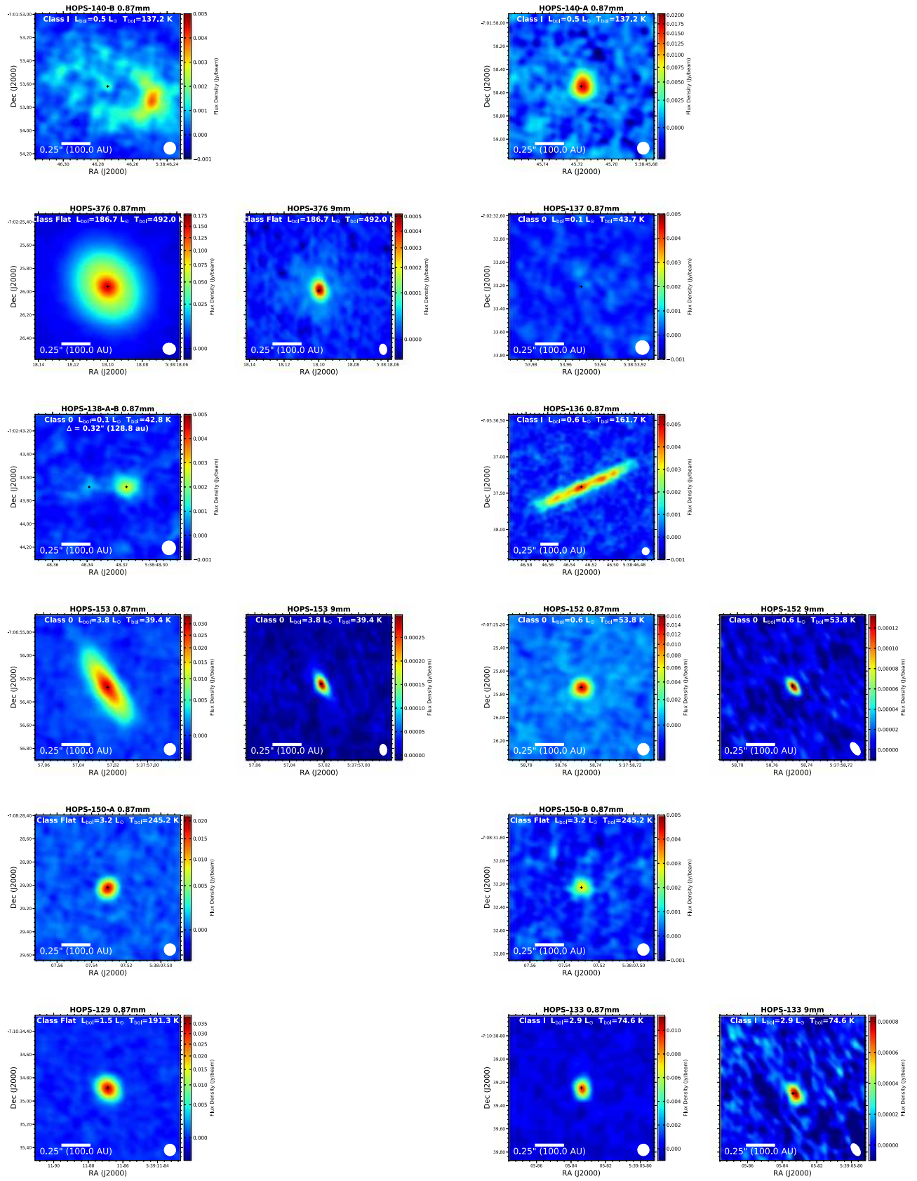
Figure 45. Orion images.
