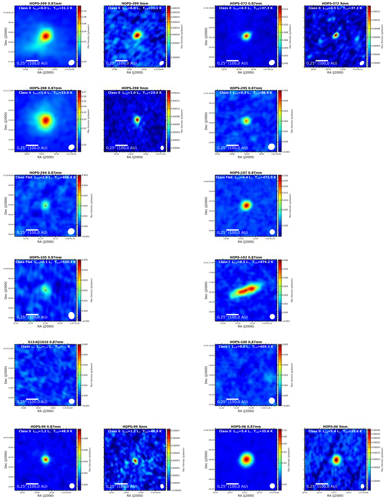
Figure 29. Orion images.
