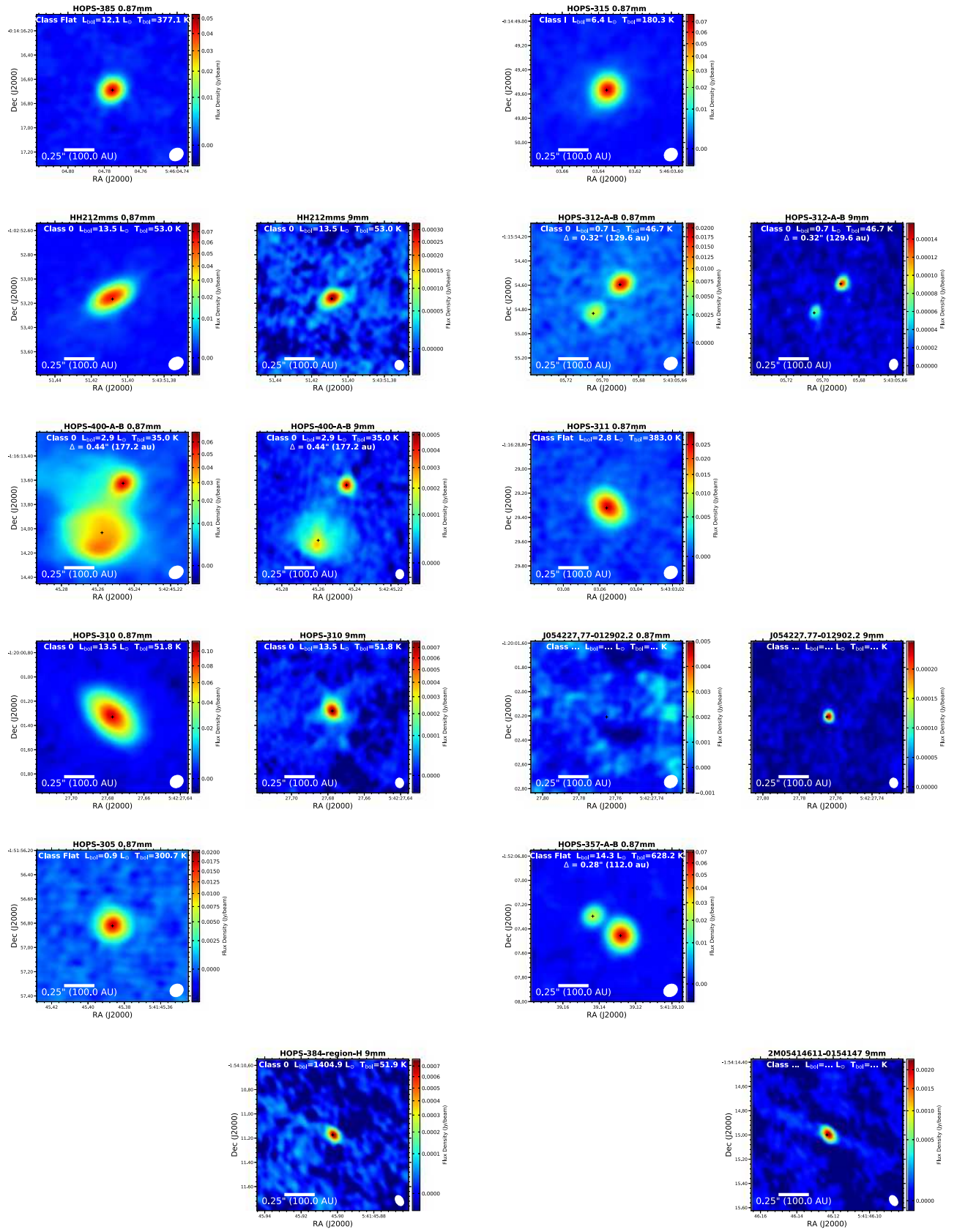
Figure 26. Orion images.
