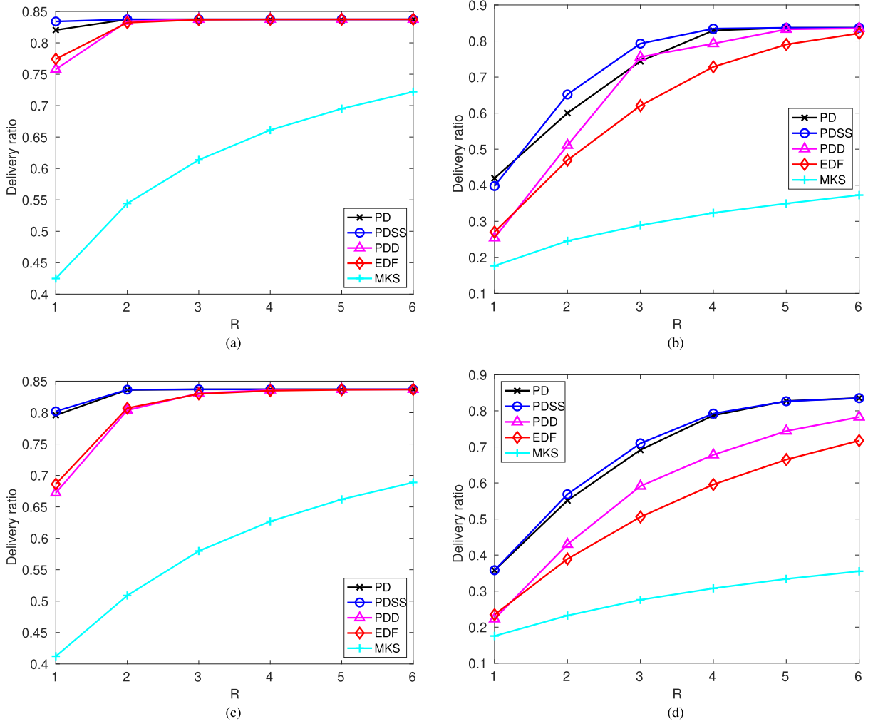
Fig. 7. Delivery ratio comparison for the 5 \times 5 grid network. (a) Homogeneous link capacity, light traffic. (b) Homogeneous link capacity, heavy traffic. (c) Heterogeneous link capacities, light traffic. (d) Heterogeneous link capacities, heavy traffic.
