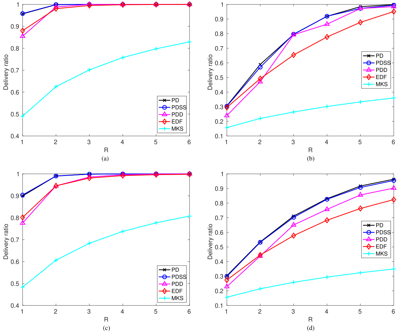
Fig. 6. Delivery ratio comparison for the small network. (a) Homogeneous link capacity, light traffic. (b) Homogeneous link capacity, heavy traffic. (c) Heterogeneous link capacities, light traffic. (d) Heterogeneous link capacities, heavy traffic.
