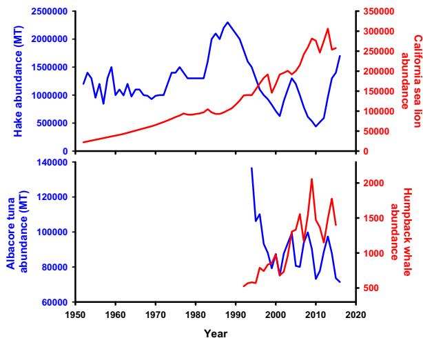
Figure 6. Population size of key top predators of CSNA, 1950–2016. Top: Pacific hake [Berger et al. 2017 (modified: total biomass divided by three to obtain biomass of age-5+ fish likely to consume CSNA)] and California sea lion [Carretta et al. , 2017; Laake et al. , 2018 (modified: 1960, 1962–1967, 1979–1980, and 2012 filled by trend analysis from surrounding years; 1958–1959, 1961, 1968–1974 imputed twice based on an average difference between Carretta et al. and Laake et al. from 1975 to 1981)]. Bottom: albacore tuna [International Scientific Committee for Tuna and Tuna-like species in the North Pacific Ocean, 2017 (modified: sum of both sexes ages 2–4 based on numbers and weight at age from the base model of the 2017 stock assessment, assuming that 40% of that biomass is in the eastern North Pacific and 56% of the eastern North Pacific biomass is found from San Francisco, United States, to Ensenada, Mexico; S. Teo, pers. comm. to SD)] and humpback whales (after Calambokidis et al. , 2017; Table 2). Fish are shown in blue, and marine mammals are shown in red.
