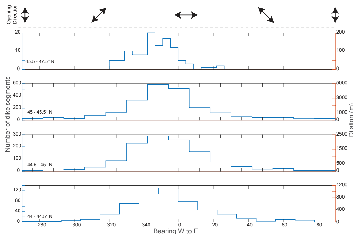
Figure 13. Dike dilation binned by bearing and latitude. Each subplot represents dikes binned initially by latitude ( 44^\circ – 44.5^\circ\text{N} ; 44.5^\circ – 45^\circ\text{N} ; 45^\circ – 45.5^\circ\text{N} ; and 45.5^\circ – 47.5^\circ\text{N} ), see Figure 2 for reference, with dilation as a function of orientation (compare with Figs. 2B and 2C for the E-W and N-S components). The right scale is the magnitude of dilation assuming an average dike width of 8 m. The opening direction is provided for reference at the top, highlighting for example that a dike oriented due N-S is actually opening E-W. Dike count and total dilation calculation is sensitive to the range of latitudes chosen to limit each histogram, but this does not affect the overall shape of the distributions.
