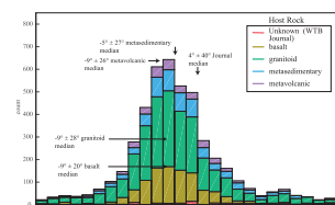
Supplementary Figure S1: Dike bearing, binned by host rock type. This plot shows the predominance of the NNW orientation and how these orientations are consistent across rock types.
