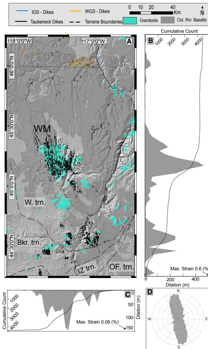
Figure 2. (A) Current mapped extent of the Chief Joseph dike swarm, as mapped predominantly by William H. Taubeneck ( n = 4279 ). Additional Columbia River Basalt Group (CRBG)-related dikes mapped by other sources are included. Dikes mapped by the Idaho Geological Survey and dikes mapped by the Washington Geological Survey (Schuster, 2005; Lewis et al., 2012; Blakely et al., 2014). Major Mesozoic and Paleozoic terrane boundaries are within the dashed lines. Abbreviations: Wallowa terrane—W. trn.; Baker terrane—Bkr. trn.; Ilee terrane—IZ trn.; Olds Ferry Terrane—OF trn. (Schwartz et al., 2014b). Columbia River Basalt flows extracted from the state geologic maps (Walker and MacLeod, 1991; Schuster, 2005; Lewis et al., 2012). (B) The thin line is a cumulative count of dike segments across the dike swarm with increasing latitude. The gray region is the calculation of minimum E-W dilation as a result of diking (see Methods section). Strain is calculated over a 350-km-long region NS, and a 100-km-wide region EW. (C) The N-S minimum component of dilation. (D) A moving average rose diagram of dike orientations (Munro and Blenkinsop, 2012).
