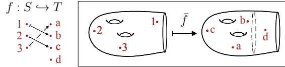
Figure 4: The FI-module structure on H_i(F(M); R) .
