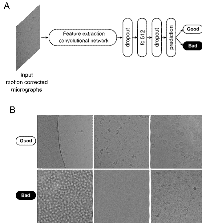
Figure 2. Deep learning-based tools for cryo-EM micrograph and 2D class average assessment. (A)
