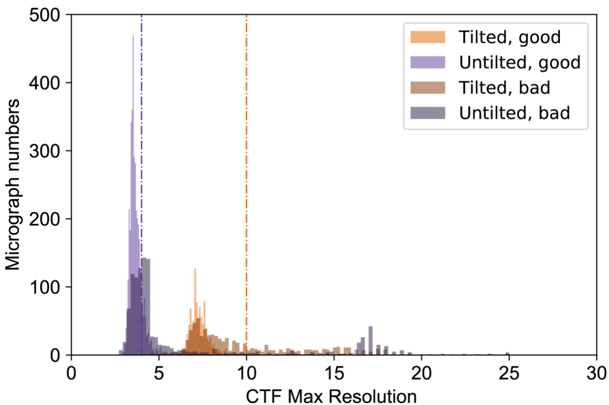
Figure S1, Related to Figure 3. Comparison of CTF maximum resolution vs. ground truth (human assessment). Histograms of the CTF maximum resolutions outputted by CTFFIND4 of the P-Rex1 test set, color labeled according to the manually labeled ground truth. Vertical lines indicate 4 Å and 10 Å respectively.
