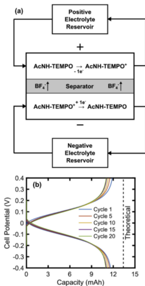
Figure 6. (a) Schematic of a symmetric flow cell during charging of a TEMPO-based molecule in non-aqueous electrolyte. (b) Potential vs. charge for selected cycles of symmetric cell cycling of 50 mM total active species in 0.5 M LiBF 4 /PC. Reprinted with permission from ref 149. Copyright 2016 Elsevier.
