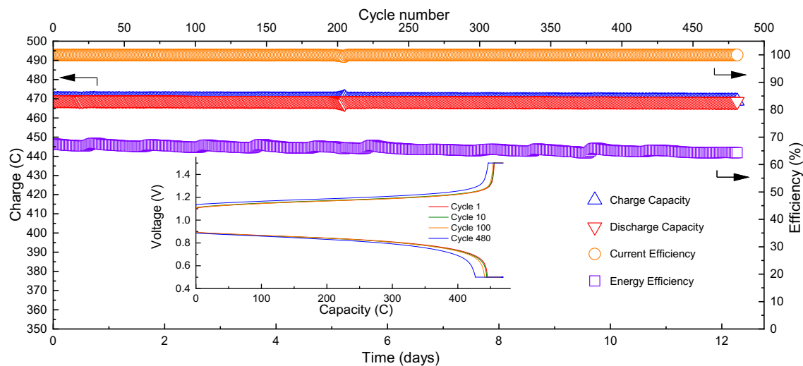
Figure 4. Current efficiency, energy efficiency, charge (upward-pointing triangles) capacity, and discharge (downward-pointing triangles) capacity versus time and cycle for a full cell comprising 5 mL 0.5 2,6-DPPEAQ at pH 9 in the negolyte, and 80 mL 0.4 M potassium ferrocyanide and 0.1 M potassium ferricyanide at pH 9 in the posolyte. The cell was cycled galvanostatically at 100 mA/cm 2 between 1.5 and 0.5 V, and each half-cycle ended with a potentiostatic hold until the magnitude of the current density fell below 2 mA/cm 2 . Inset: capacity versus cell voltage at the 1 st , 10 th , 100 th and 480 th cycle. Adapted with permission from ref 54. Copyright 2019 John Wiley and Sons.
