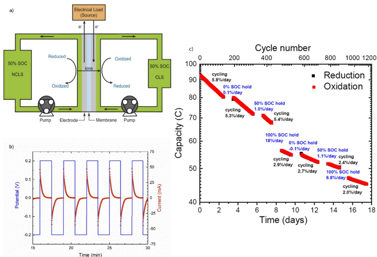
Figure 7. (a) Schematic of unbalanced, compositionally-symmetric flow cell. (b) Example of symmetric cell potentiostatic cycling protocol. (c) Semi-log plot of unbalanced, compositionally-symmetric cell cycling of 50% SOC 0.1 M DHAQ in 1 M KOH with cycling pauses at different SOC levels. Temporal capacity fade rates from slopes of each cycling segment are denoted in black text. Capacity loss and SOC of CLS during 24-hour pauses are denoted in blue text. Reprinted with permission from ref 33. Copyright 2018 Electrochemical Society.
