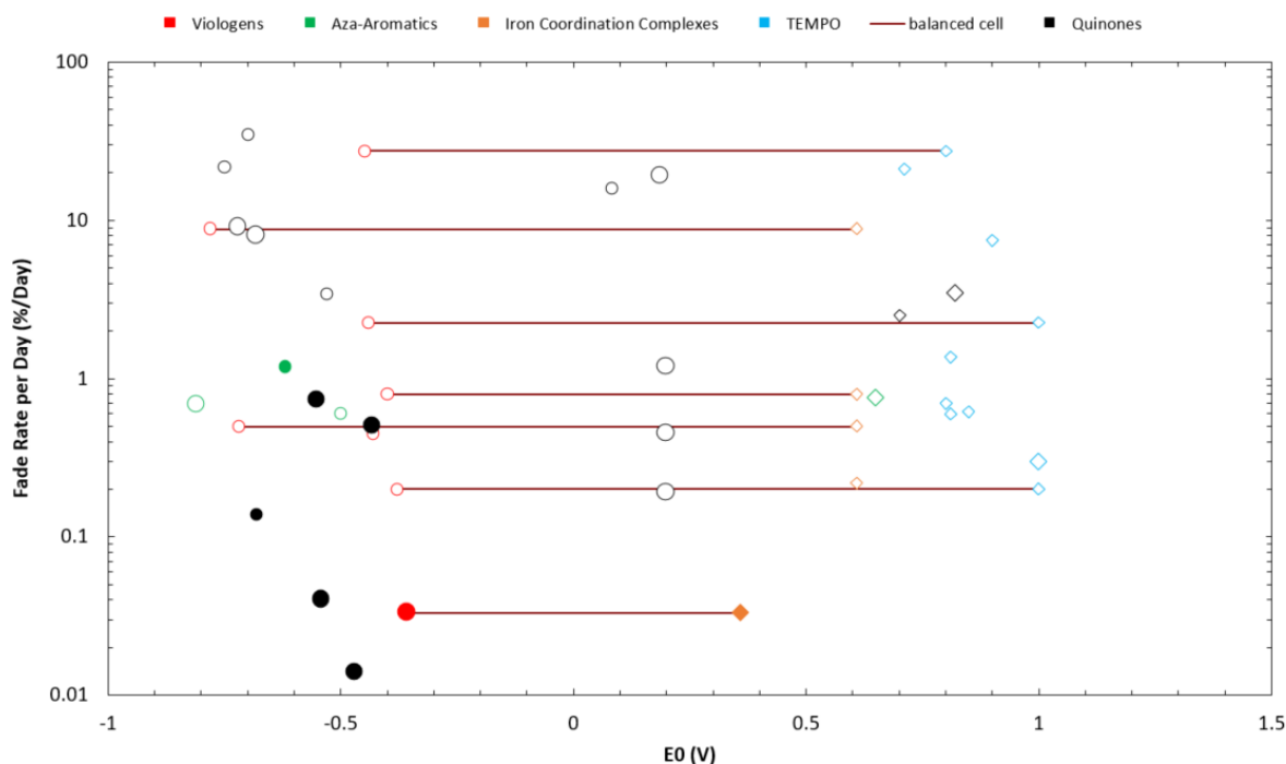
Figure 8. Plot showing full cell capacity fade rate in %/day vs redox potential (vs SHE) for viologen (red), aza-aromatic (green), iron coordination complex (orange), TEMPO (blue) and quinone (black)-based chemistries. Posolytes are indicated using diamonds, and negolytes in circles, whereas points depicting chemistries with electron concentrations \geq 1.0 M are larger than those < 1.0 M. Points depicting capacity fade results of chemistries that have been tested using potentiostatic or combined potentiostatic-galvanostatic cycling have been filled, whereas those depicting apparent capacity fade results obtained with only galvanostatic cycling have been left empty. Capacity-balanced cells where both sides contain organics/organometallics are marked out with a horizontal line connecting negolyte and posolyte chemistries.
