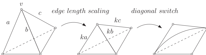
FIG. 1. Discrete conformal change of PL metrics. All triangulations are Delaunay
