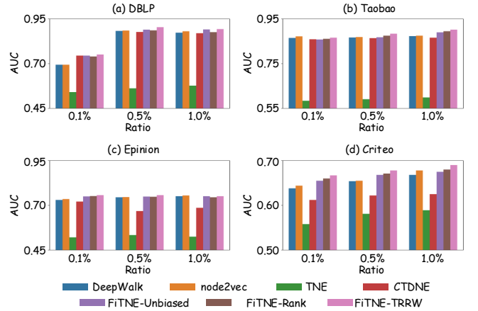
Figure 4: Link prediction results (AUC) with different ratios of sampled edges.
