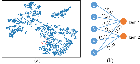
Figure 5: (a) Visualization of embedding representations generated from Criteo using t-SNE; (b) Visualization of the mininature consists of nodes marked in Fig. 5(a). The timesamp and time duration of the edge are labeled on the edge.
