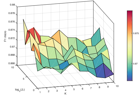
Figure 6: Hyperparameter analysis on Taobao.
