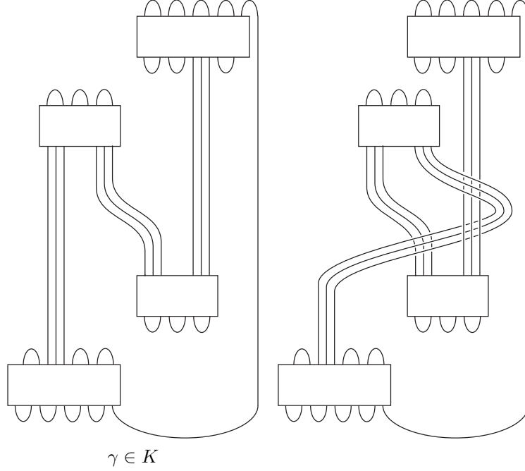
Figure 3. K \in \mathcal{K} and K \# K_2
