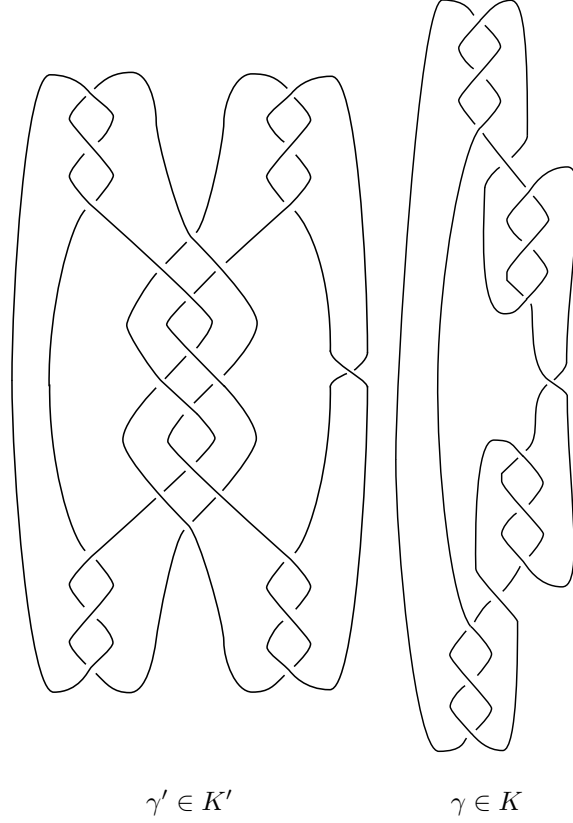
Figure 2. A counterexample for Theorem 4.2 without the condition w(K) = w(K')
