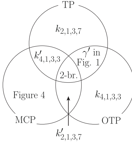
Figure 5. Venn diagram for TP, MCP and OTP
