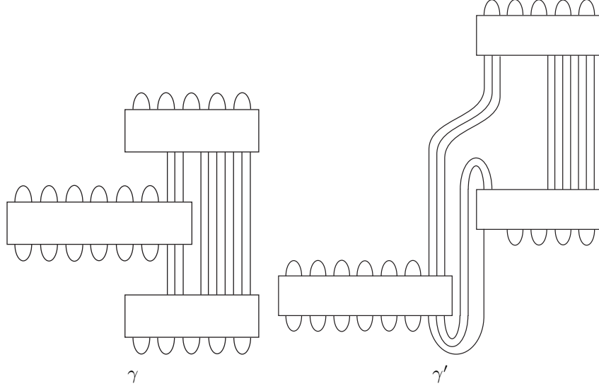
Figure 1. A potential example for Conjecture 2.3, where w(\gamma) = w(\gamma') = 242 .
