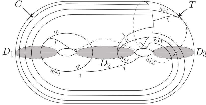
Figure 6. Constructing a knot K with r(F, K) \geq n which bounds an essential once punctured Klein bottle
