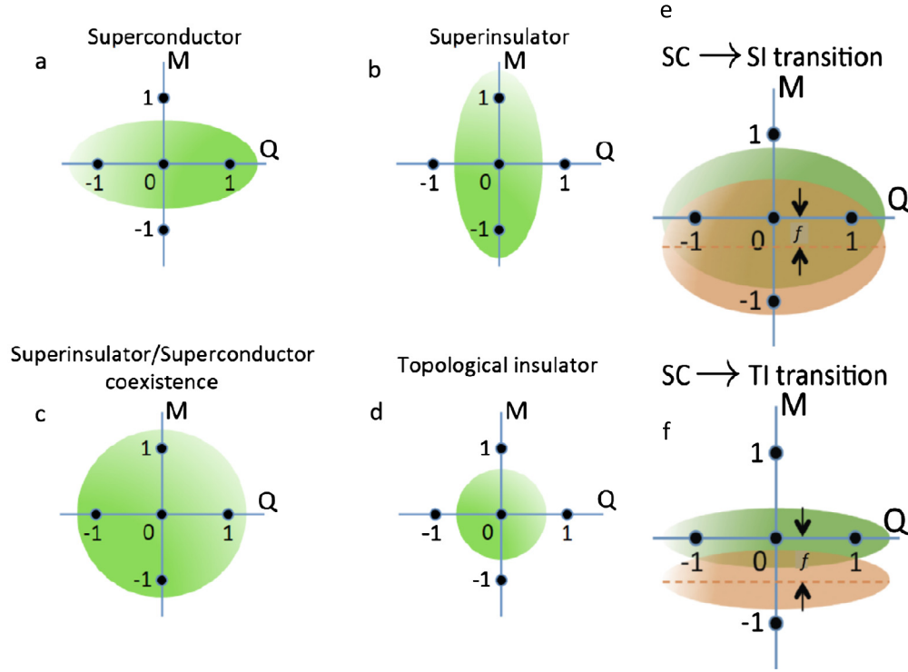
Fig. 2. Graphic representation of the conditions for realizing different phases near the SIT. a: Superconductor: Strings with electric quantum numbers condense. b: Superinsulator: Strings with magnetic quantum numbers condense. c: Coexistence of long electric and magnetic strings near the first-order direct transition from a superconductor to a superinsulator. d: Bosonic topological insulator/Bose metal: all strings are suppressed by their high self-energy. e: Phase transitions induced by an external magnetic field: Direct, magnetic-field-induced transition from a superconductor to a superinsulator for \eta < 1 . f: Magnetic-field-driven transition from a superconductor to a topological insulator for \eta > 1 .
