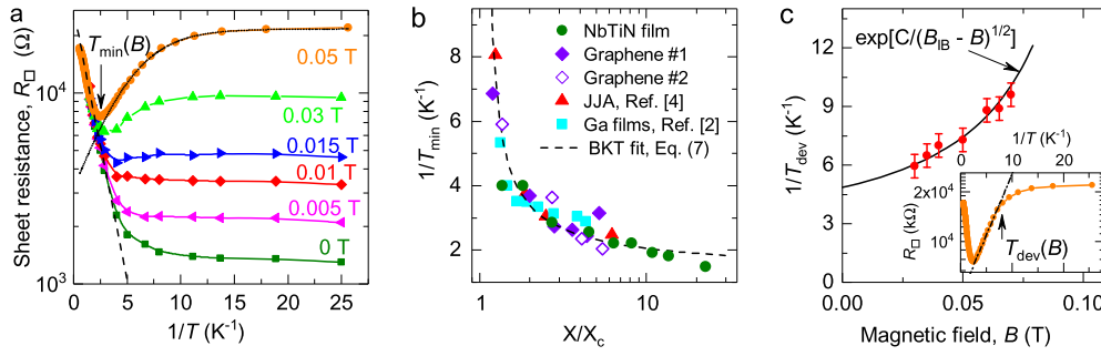
Fig. 5. Sheet resistance vs 1/T plots and the BKT scaling for correlation lengths. a: Representative \log R_{\square} vs. 1/T plots. The dashed black line depicts R \propto \exp(-T^*/T) dependence. The dotted line describes R_{\square}(1/T) behavior for two parallel resistors comprising R_b \propto \exp(T^{**}/T) (bulk modes) insulating dependence and constant (edge ballistic modes) behavior, see text. b: The BKT scaling of 1/T_{\min} \sim \xi_{\text{corr}} \sim \exp[\text{const}/(X/X_c - 1)^{1/2}] of the BKT correlation length near the superconductor-BM quantum BKT transition in different materials driven by either magnetic field, disorder, or gate voltage, demonstrating the universality of the BKT superconductor-BM transition. The circles stand for T_{\min}(B) in NbTiN films, X/X_c = B/B_{SB} ; the diamonds mark data for Van der Waals heterostructures of twisted double bilayer graphene (TDBG) where the SIT is tuned by the in-plane magnetic field, X/X_c = B_{\parallel}/B_c , B_c = 2.5 T is an adjustment parameter and T_{\min} is divided by 35; the triangles mark data for the SIT driven by the frustration factor f = \Phi/\Phi_0 , with \Phi being the magnetic flux per plaquette in JJA, f_c = 0.1 [4], and squares mark the film thickness driven SIT in granular films [2], for which X/X_c = R_N/R_{NC} , R_{NC} = 32 kΩ, T_{\min} is divided by 16. c: The BKT scaling of the correlation length \sim 1/T_{\text{dev}} near the insulator-Bose metal transition, detected by deviation of the resistance from the exponential insulating \exp(T^{**}/T) behavior (the dashed line in the inset).
