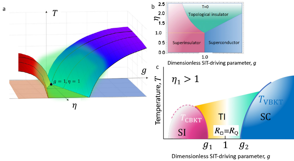
Fig. 3. Phase structure of the SIT. a: Three-dimensional sketch of the phase diagram near the SIT in (g, \eta, T) coordinates. The red and blue surfaces represent the loci for charge and vortex BKT transitions, the green “cloud” depicts the domain of the Bose metal, which is shown (see text) to be a bosonic topological insulator, hence marked as TI. b: Zero temperature cut of the phase diagram. c: A cut at \eta > 1 , representing the schematic phase diagram for strong quantum fluctuations (not to scale) near the SIT. The topological insulator (TI) state is separated from the superconducting (SC) and superinsulating (SI) states by vortex- and charge-BKT transitions respectively (magenta and blue solid lines respectively). In the vicinity of the T_{VBKT} line, R_{\square} < R_Q and the system exhibits metallic behavior which crosses over smoothly into the thermally activated insulating behavior upon decreasing g shown by the change of the color. At g = 1 , R_{\square} = R_Q and the resistance keeps increasing, R_{\square} > R_Q , towards the T_{CBKT} line. The yellow strip depicts the domain of thermally activated resistance, which crosses over to BKT critical behavior on approach to T_{CBKT} . The SIT-driving values g_1 and g_2 that mark superinsulator-Bose metal and superinsulator-Bose metal quantum transitions satisfy the duality relation g_2 = 1/g_1 . The parameter g can be either the dimensionless conductance of the film, or magnetic field, or gate voltage in the gate-driven SIT.
