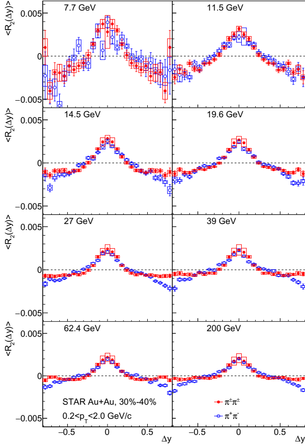
(a) pions
