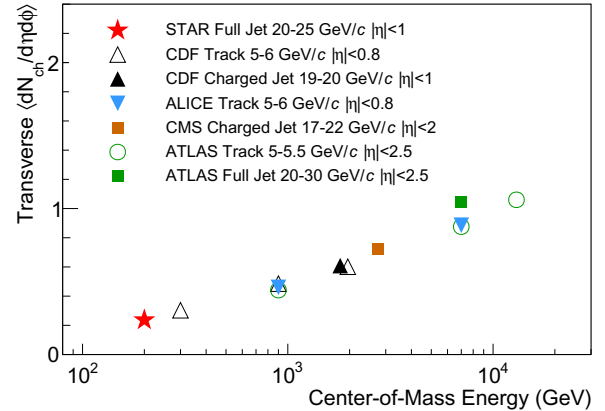
FIG. 7. Transverse charged particle densities at various center-of-mass collision energies. Uncertainties smaller than the marker sizes. See text for details.
