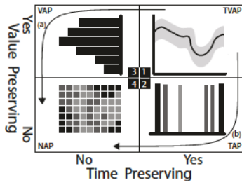
Figure 2: Periphery plot types can be characterized by their preservation of the time and value axes. Summarization can prioritize (a) value preservation or (b) time preservation.
