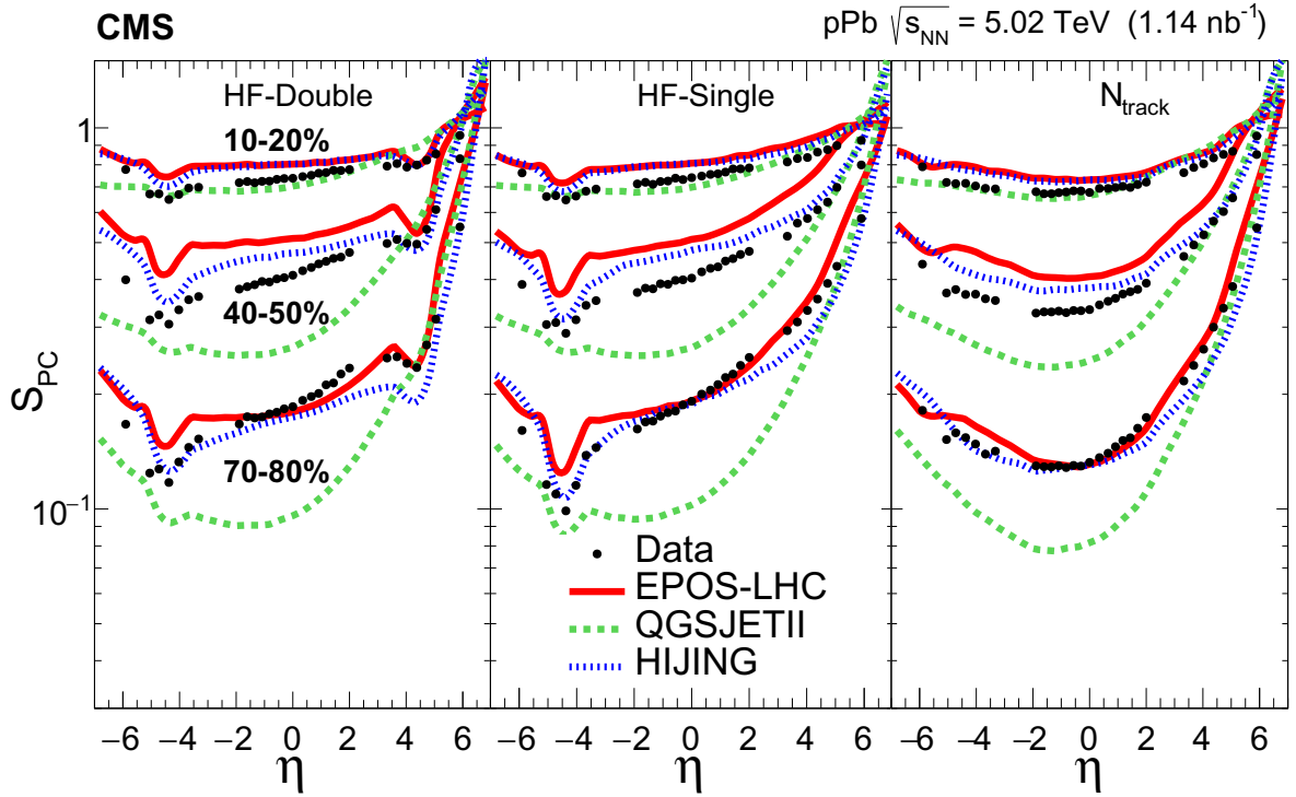
Figure 5: Ratio of peripheral to central E_T production, S_{\text{PC}} , as a function of \eta for three centrality ranges for HF-Double (left), HF-Single (middle), and N_{\text{track}} (right) for data, and for the EPOS-LHC, QGSJET II, and HIJING event generators. The systematic uncertainties are dominant and are of comparable size to the data points.
