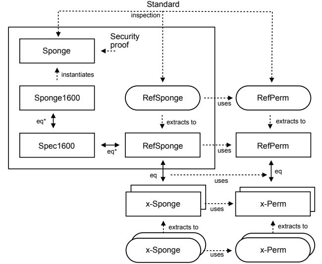
Figure 14: Equivalence proofs
