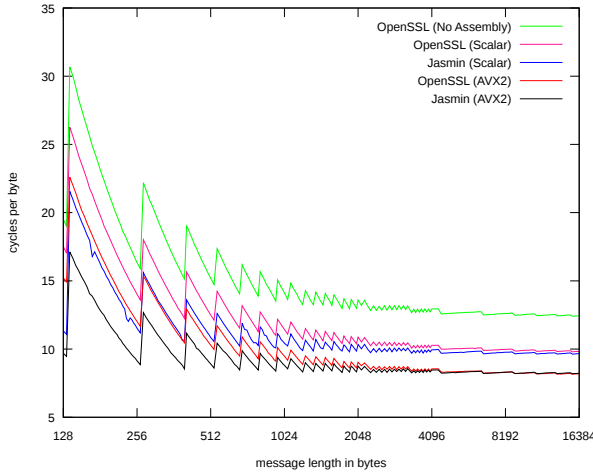
Figure 15: Comparison to non-verified code.
