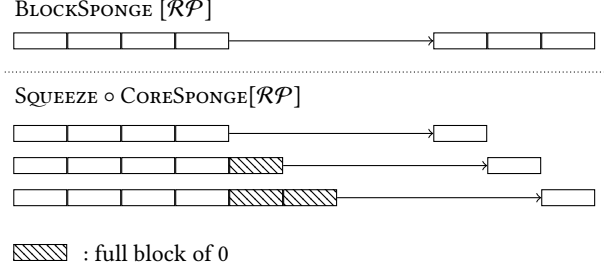
Figure 6: BLOCKSPONGE [\mathcal{RP}] and SQUEEZE \circ CORESPONGE [\mathcal{RP}] on inputs that are a list of 4 blocks and output size 3.
