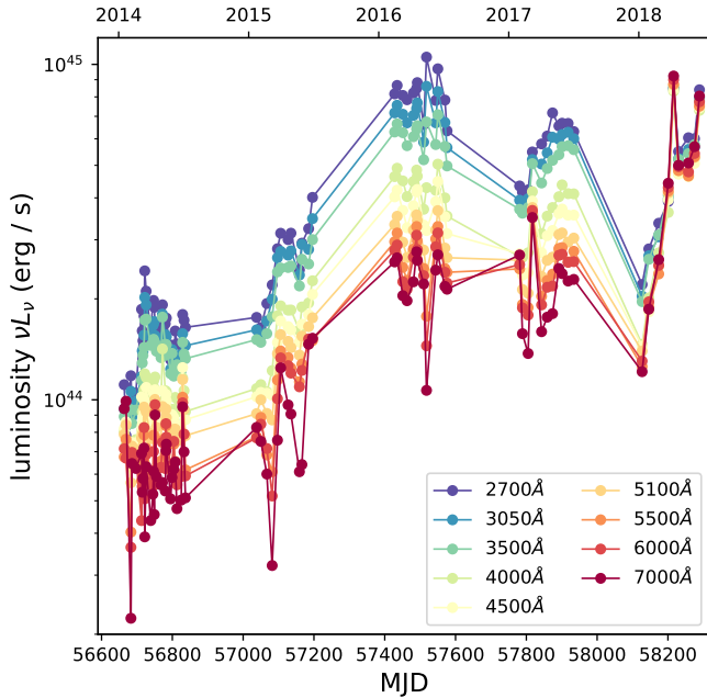
Figure 2. Host galaxy subtracted, rest frame multi-band continuum light curves measured from the SDSS spectra. During the initial large rise the continuum maintains a blue shape. In the later drop and sharp rise in 2018 it suddenly reddens. At the final peak, the SED is completely flat across the observed optical range. The host galaxy dominates in the red bands ( \lambda \gtrsim 4000\text{\AA} ) in 2014-2015 when the AGN optical luminosity is low ( L \lesssim 10^{44} \text{ erg s}^{-1} , Shen et al. 2015b).
