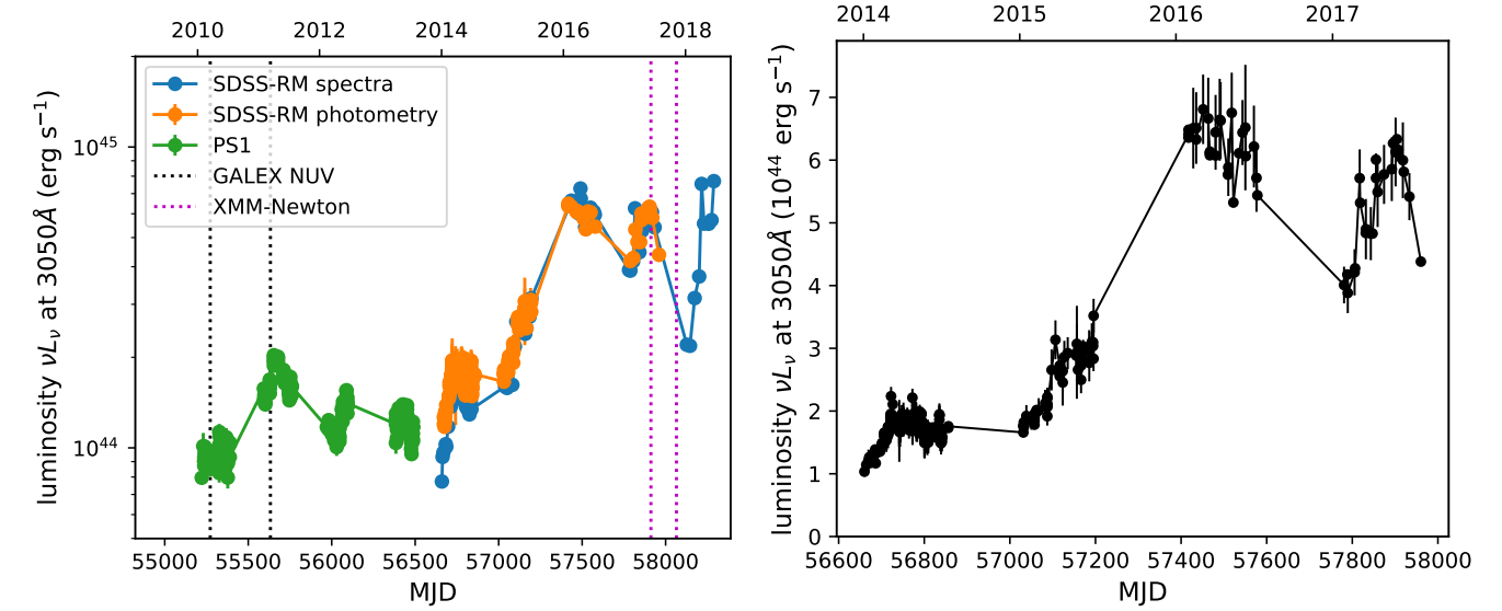
Figure 1. Continuum optical light curve for SDSS J141324+530527 from 2010-2018 (left). The green and orange points are luminosities derived from Pan-STARRS PS1 and SDSS-RM g -band photometry, while the blue points are continuum measurements in the rest frame 3050Å band defined in Table 1. The dotted curves mark the extrema used to measure SEDs including GALEX NUV data, and the epochs of the XMM-Newton observations. The light curve shows continuous, rapid, large-amplitude variability. Features include a prominent rise and fall by a factor of 2 from 2010-2012, followed by a dramatic rise by almost an order of magnitude over a year from 2015-2016, and a sharp dip and final peak in 2018. In 2018 the optical luminosity increased by a factor of 3-6 in only 6 months. A zoom in of the 2014-2017 merged light curve is shown in the right panel on a linear scale.
