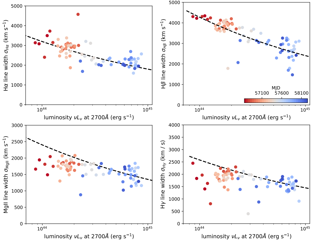
Figure 7. Line width measurements for H \alpha , H \beta , H \gamma , and MgII as a function of continuum optical luminosity. Point color indicates observational epoch (red early to blue late). The H \alpha and H \beta widths are clearly anti-correlated with luminosity. The same trend is found for MgII and H \gamma , but with a weaker dependence. The dashed curve is a relation \sigma \sim L^p with p = -1/4 , expected if the BLR radius R_{\text{BLR}} \sim L^{1/2} and radial velocity v \sim R^{-1/2} . The consistency of this trend with the data demonstrates the expected “breathing” of the BLR in response to continuum variations.
