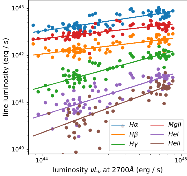
Figure 8. Line vs. 2700Å rest frame continuum luminosity for all broad emission lines measured. The solid lines are power law fits. Line luminosity is correlated with that of the continuum, but with a sub-linear slope especially for the low-ionization Balmer and MgII lines.
