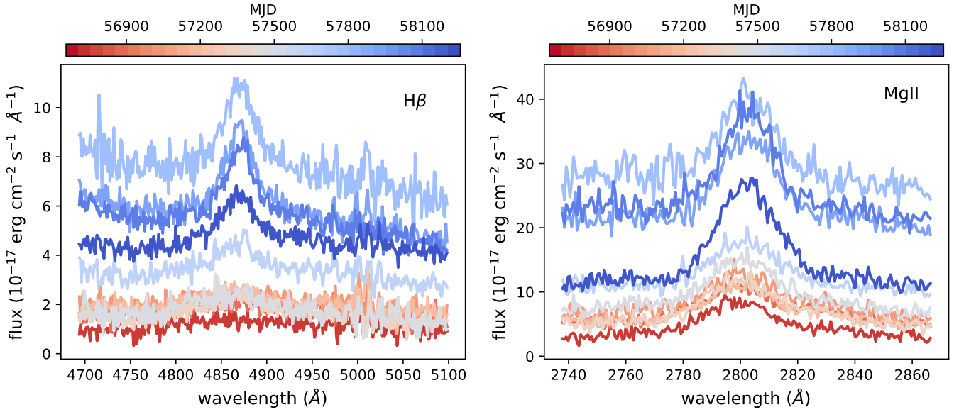
Figure 5. Sample host galaxy and narrow line subtracted H\beta (left) and MgII (right) profiles from early (red) to blue (late) epochs. The line becomes significantly narrower at late times where the continuum luminosity is higher. The shape also changes, with the core brightening more than the wings.
