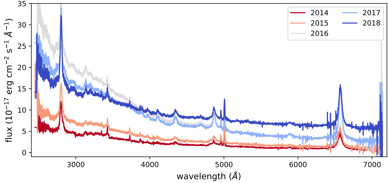
Figure 4. Host galaxy subtracted spectra averaged over each observing season. The continuum luminosity and shape change dramatically between years.
