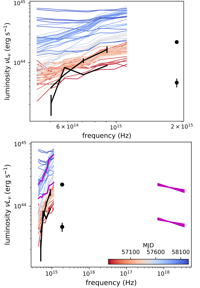
Figure 3. Host galaxy subtracted, rest frame, optical to X-ray SEDs. The black curves and points show quasi-simultaneous PS1 and GALEX photometry. The magenta curves show quasi-simultaneous continuum measurements from SDSS spectra along with XMM-Newton data. The colored curves are measurements from SDSS-RM spectra going from early (red) to mid (gray) to late (blue) epochs. The optical SEDs are consistent with power laws. In the lower state, the SED peak appears to be redwards of the GALEX NUV point. In the GALEX higher state and most of the SDSS-RM spectra, the peak is bluewards of our observing band. Where measured, the X-ray luminosity is relatively high but well below that of the bluest optical band. During the dramatic rise in 2018, the SED reddens to become completely flat across the optical band.
