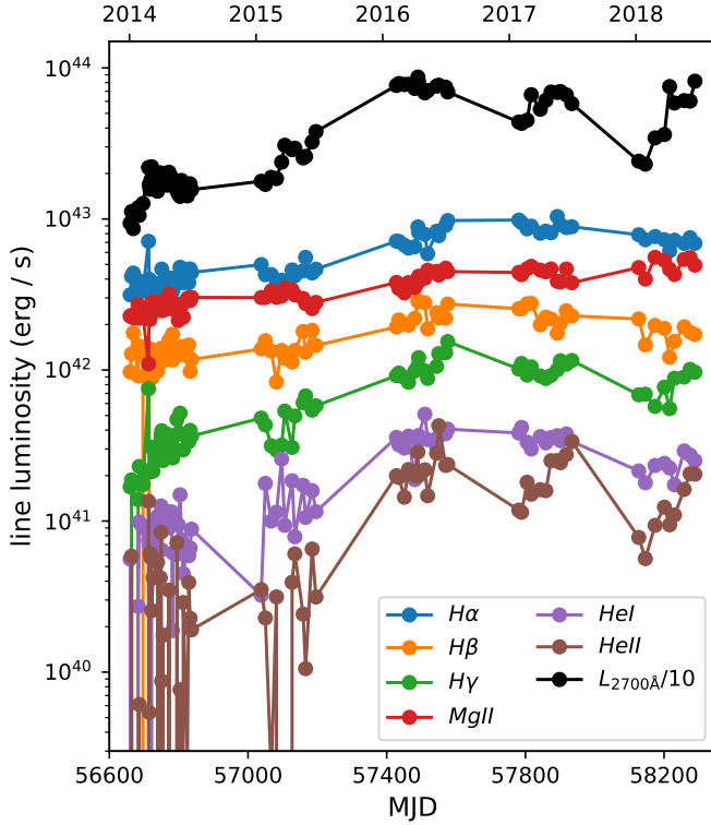
Figure 6. Continuum and broad emission line light curves measured from the SDSS spectra. All lines increase in luminosity during the large rise in the optical continuum. The He lines show a stronger response than the Balmer and MgII lines.
