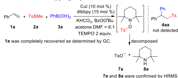
Scheme 3. Control Experiments to Probe the Reaction Mechanism.
