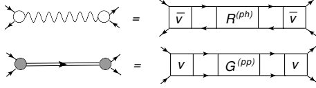
Figure 2. Diagrammatic mapping of the EOM to the PVC-TBA. Empty and filled circles denote the coupling vertices of the normal and pairing phonons, respectively, and the wiggly and double lines their propagators. R^{(ph)} and G^{(pp)} are the particle-hole response function and the particle-particle Green function, respectively.
