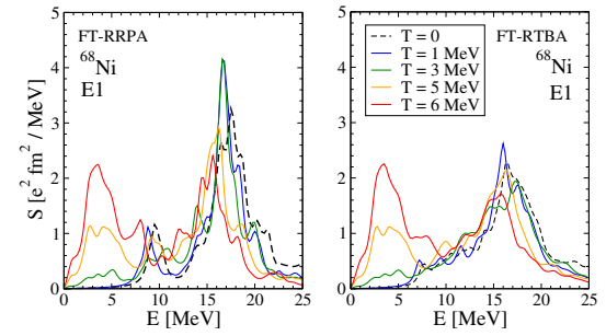
Figure 5. Dipole strength distribution in 68 Ni at various temperatures in the finite-temperature relativistic RPA (FT-RRPA) and in the finite-temperature relativistic time blocking approximation (FT-RTBA).
