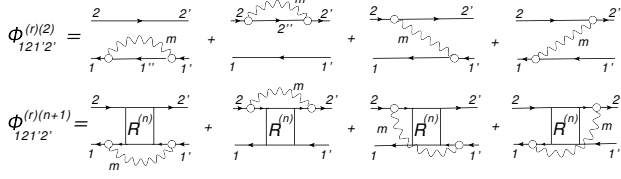
Figure 3. Dynamical kernel of the conventional PVC-TBA (top) and generalized EOM-TBA (bottom).
