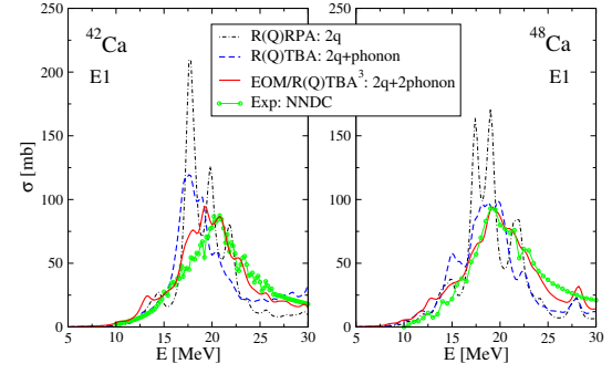
Figure 4. Theoretical dipole photoabsorption cross sections in 42,48 Ca compared to the evaluated experimental data of Refs. [45, 46].
