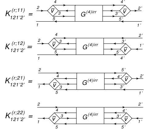
Figure 1. The components of the dynamical kernel K_{12,1'2'}^{(r)}(t-t') . Straight solid lines stand for fermionic propagators, the square blocks denote the antisymmetrized nucleon-nucleon interaction \bar{v} , and the rectangular blocks G^{(4)} correspond to the two-particle-two-hole Green function (7).
