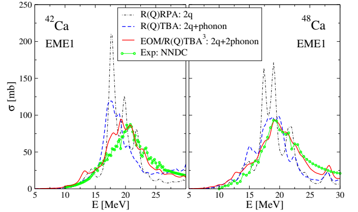
FIG. 16. Giant dipole resonance in ^{42,48}\text{Ca} nuclei calculated within R(Q)RPA, R(Q)TBA and EOM/R(Q)TBA 3 with \Delta = 500 keV, in comparison to experimental data of Ref. [83, 95].
