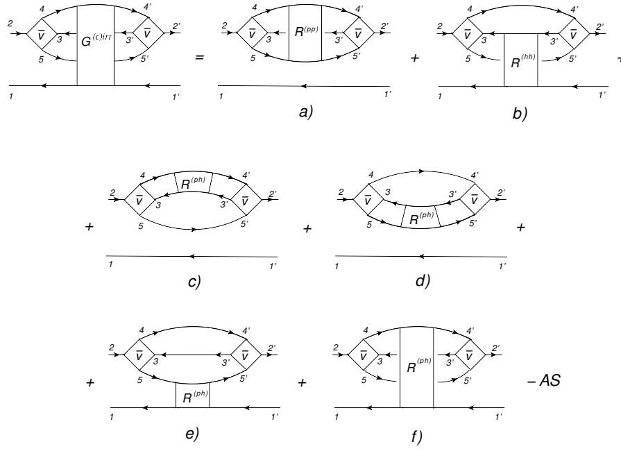
FIG. 7. Diagrammatic representation of the singly correlated approximation of Eq. (90) to the dynamical kernel K_{12,1'2'}^{(r;11)}(t-t') irreducible with respect to the particle-hole propagator. "AS" includes the antisymmetrized contributions, similar to that of the uncorrelated part, Fig. 6.
