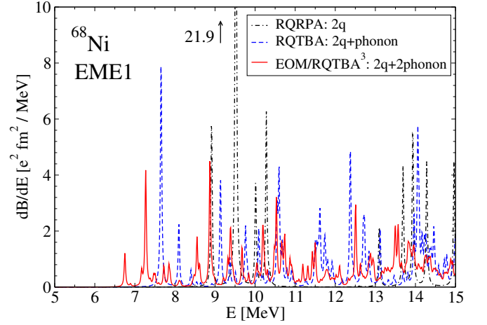
FIG. 18. The low-energy dipole spectrum S(E) = dB(E)/dE of ^{68}\text{Ni} nucleus calculated within RQRPA, RQTBA and EOM/RQTBA 3 with \Delta = 20 keV.
