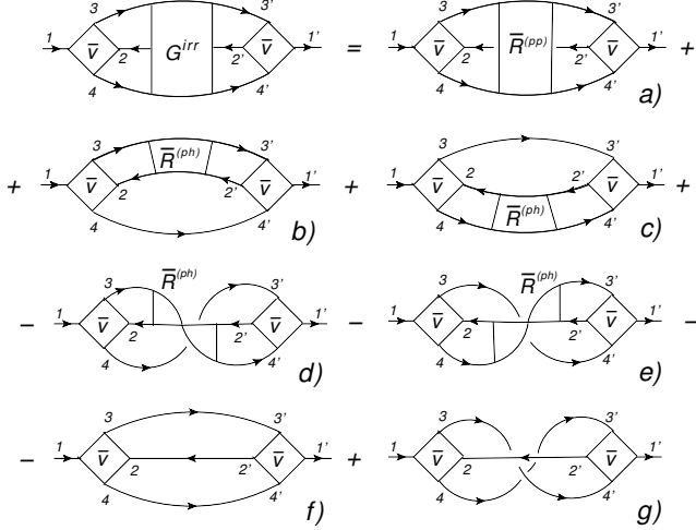
FIG. 1. Diagrammatic representation of the dynamical self-energy \Sigma^{(r)} of Eq. (46) in terms of the uncorrelated one-fermion (lines with arrows) and correlated two-fermion (boxes \bar{R} together with long lines with arrows) intermediate propagators. Blocks \bar{v} stand for the bare two-fermion interaction.
