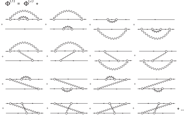
FIG. 14. The simplest time-ordered 2q \otimes 2\text{phonon} diagrams taken into account in EOM/RQTBA 3 . The ellipsis stands for multiple PVC exchange and self-energy contributions as well as for the correlated particle-hole configurations in the internal particle-hole propagators.
