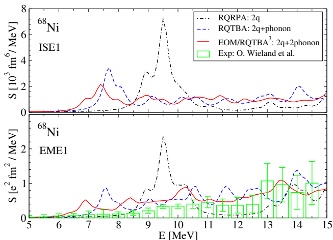
FIG. 19. The low-energy dipole spectrum of ^{68}\text{Ni} nucleus calculated within RQRPA, RQTBA and EOM/RQTBA 3 with \Delta = 200 keV. Top: the isoscalar dipole strength distribution, bottom: the electromagnetic dipole strength distribution in comparison to experimental data of Ref. [108].
