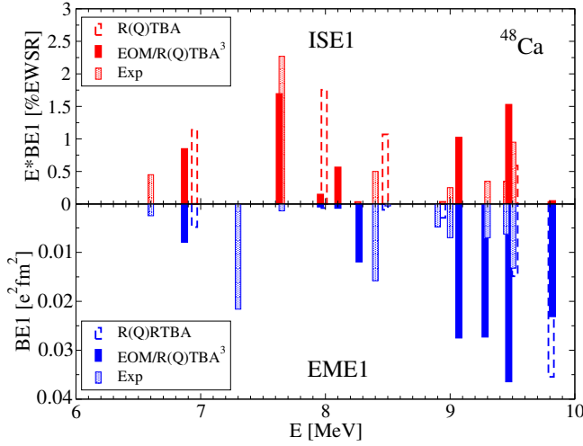
FIG. 17. The low-energy dipole strength of ^{48}\text{Ca} nucleus calculated within R(Q)RPA, R(Q)TBA and EOM/R(Q)TBA 3 . The reduced transition probabilities are shown for the isoscalar (top) and electromagnetic (bottom) dipole operators in comparison to experimental data of Ref. [103].
