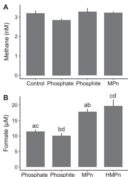
FIG 2 Methane and formate produced by Prochlorococcus strain MIT9301 grown with phosphate, phosphite, methylphosphonate (MPn), or hydroxymethylphosphonate (HMPn). (A) Dissolved methane concentrations measured in MIT9301 cultures after 7 days of growth in gas-tight bottles. The control measurement corresponds to the methane concentration at the start of the incubation to account for the solubility of atmospheric methane in the medium. The error bars represent the standard deviations of the means from triplicate cultures. (B) Formate concentrations measured in the supernatant of MIT9301 cultures grown to maximum cell densities for 14 days with the indicated P substrate as sole P source. Formate was not detected in the sterile medium at the start of the incubation. Error bars represent the standard deviations of the means from triplicate cultures. The average formate concentrations in treatments marked with the same lowercase letter (a, b, c, or d) were significantly different ( P < 0.05 ).
