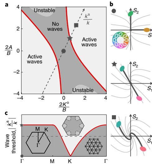
Fig. 5 | Exceptional points and non-Hermitian elastodynamics. a , Phase diagram for waves in an overdamped odd-elastic solid. The red curves represent the boundary outside of which active waves can be sustained. b , The eigenmodes for three relative values of the elastic moduli, showing trajectories in shear space ( S_1 and S_2 , Fig. 4). At zero activity (circle symbol), the modes correspond to longitudinal and transverse waves, whose eigenvectors are orthogonal in S_1 - S_2 space. At the exceptional point (star symbol), the eigenmodes become co-linear. Above the exceptional point (square symbol), the eigenmodes acquire a circular polarization, performing a spiral through simultaneous rotation and attenuation in strain space. See Supplementary Video 4. c , A cut ( \Gamma MK \Gamma ) through the space of wavevectors (first Brillouin zone) of a triangular lattice with generalized Hookean springs. The microscopic activity in the springs is characterized by the ratio |k^a/k| between odd spring constant k^a and conservative spring constant k . The threshold for active waves varies across the Brillouin zone, with the elastic limit describing the region near \Gamma . The middle inset shows the regions of the Brillouin zone (light grey) in which waves propagate (for |k^a/k| corresponding to the horizontal dashed line).
