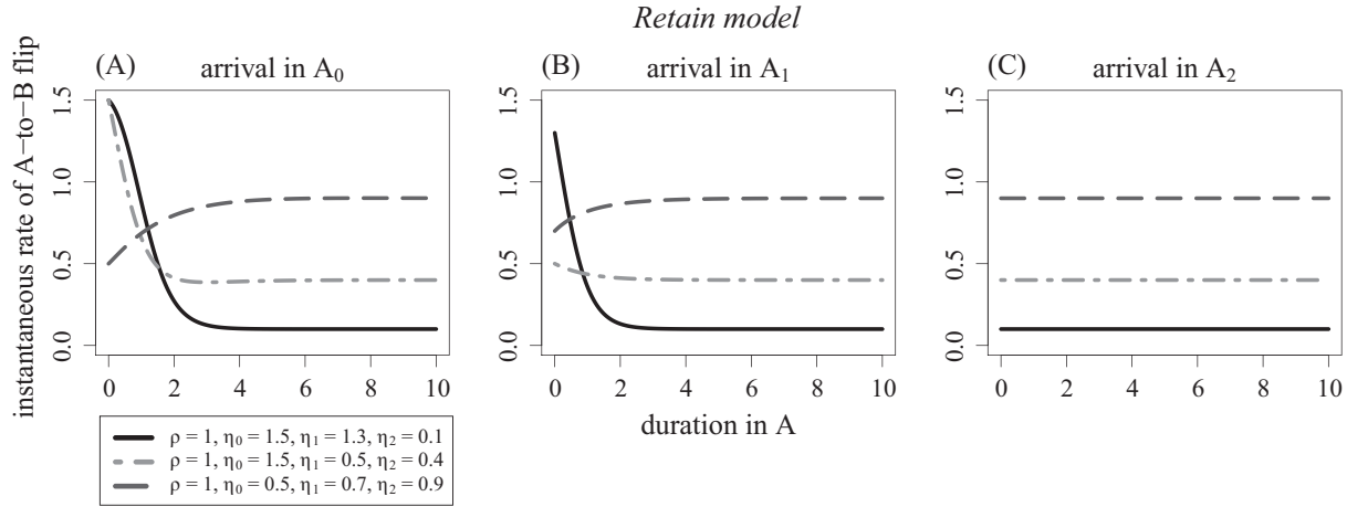
Figure 4: Hazard functions for the retain model. For the scenario in which adaptation subtraits are retained upon a flip in the focal trait (fig. 2C), the rate of flips to state B depends on whether the initial substate was A_0 (A), A_1 (B), or A_2 (C). This precludes the use of a two-state renewal process framework.
