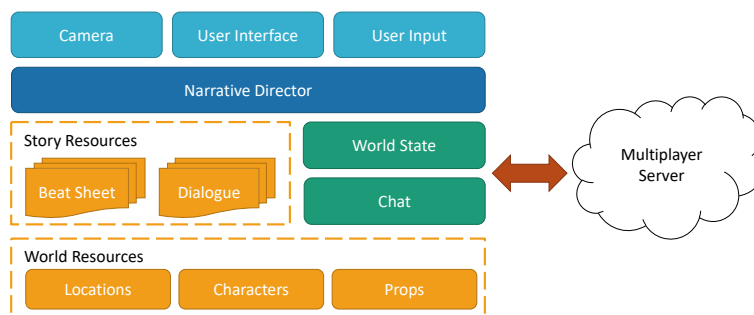
Fig. 1. STORYLOOM architecture.
