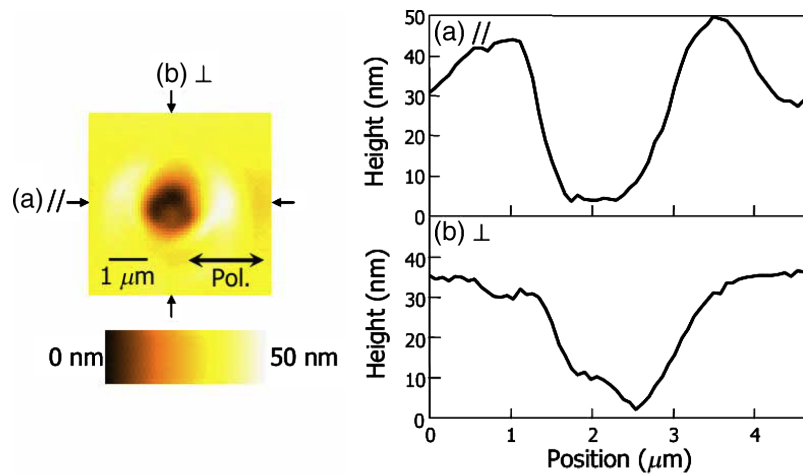
Fig. 13 Two-photon absorption-induced surface relief formed on an azopolymer film by irradiation of 920-nm femtosecond laser. (a), (b) Line plots of the relief along the parallel and perpendicular direction to light polarization. Reproduced with permission. 81 Copyright 2008, The Optical Society.
