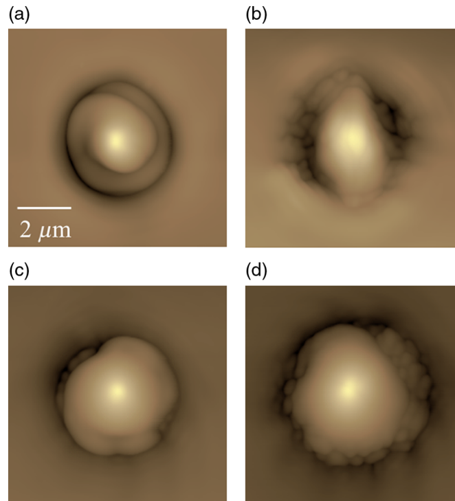
Fig. 10 Helical surface relief with a micron-scale depth. (a) and (b) Surface reliefs formed by irradiation of orbital AM beam with J = 2 ( \ell = 1 , s = 1 ) and J = 2 ( \ell = 2 , s = 0 ) respectively. (c), (d) Surface reliefs formed by orbital AM beam with J = 0 ( \ell = 1 , s = -1 ) and J = 0 ( \ell = -1 , s = 1 ), respectively. Reproduced with permission. 52 Copyright 2014, Springer Nature.
