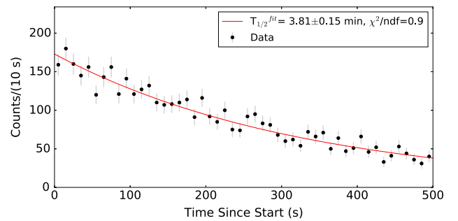
FIG. 6. Time distribution of selected SS events (black) with energies between 1075 and 4175 keV. The exponential fit is shown as red solid line.
