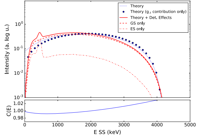
FIG. 2. (Top frame) Theoretical GS spectrum (blue dotted line) and reconstructed MC SS spectrum (red solid line). The theoretical GS spectrum shape is the same for all reasonable g_A and mesonic enhancements within the line width. The g_A -dependent contribution to the theoretical spectrum is also shown as blue dots. Individual contributions of GS and ES decays to the reconstructed spectrum are also shown as red dashed and dash-dotted lines, respectively. (Bottom frame) Shape factor, C(E) .
