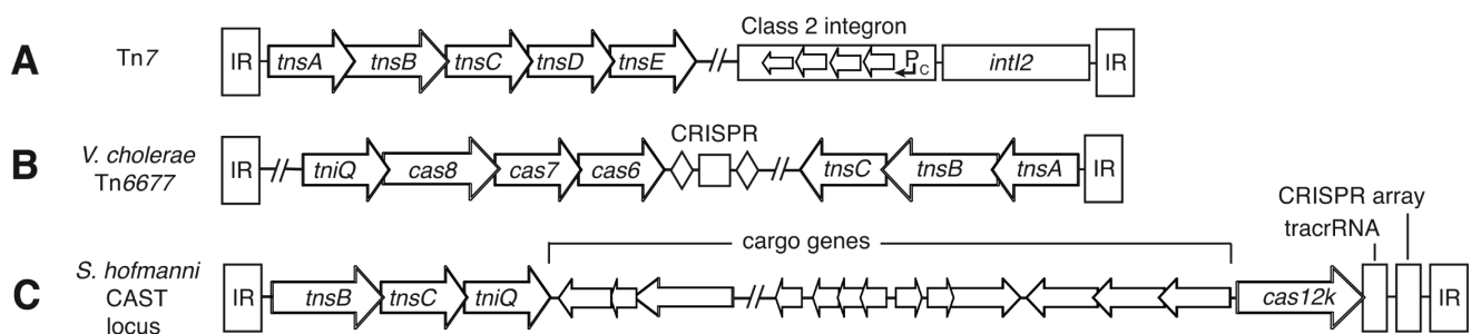
Figure 2. Sequence structure of the Tn7 transposon and derivatives encompassing clustered regularly interspaced palindromic repeats (CRISPR)–Cas-type systems. A) The structure of a typical Tn7 transposon is shown, with terminal inverted repeats (IR) shown as boxes and constituent genes shown as arrows. The diagram is based on the structure of the Escherichia coli R721 shufflon. B) The structure of the Vibrio cholerae Tn6677 transposon is shown. Tn7-derived elements and the CRISPR array are indicated. C) A representation of the Scytonema hofmanni CAST locus is provided, encompassing Tn7-like open reading frames, the effector Cas12k, and the CRISPR array. The loci are not drawn to scale.
