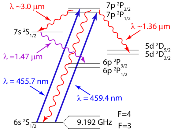
FIG. 2. Plot of the energy levels of cesium relevant to the measurements of the lifetimes of the 7p^2P_J states. We excite the 7p^2P_{3/2} ( 7p^2P_{1/2} ) state using a diode laser tuned to 455.7 nm (459.4 nm). The 7p^2P_J state can spontaneously decay to the 6s^2S_{1/2} ground state or the excited 7s^2S_{1/2} or 5d^2D_{J'} states (red wavy lines). We collect the 1.47- \mu m fluorescence from 7s^2S_{1/2} \rightarrow 6p^2P_{3/2} decay (purple wavy line).
