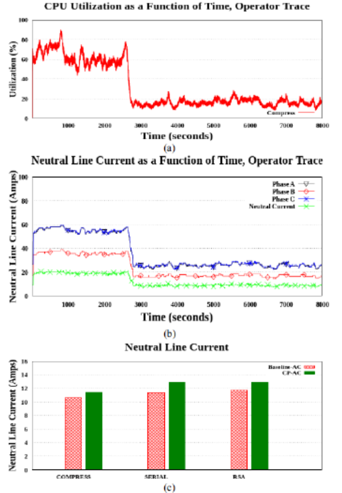
Fig. 4. Utilization and Power consumption and Neutral line Current in AC powered three phase power distribution system
