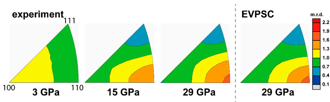
Figure 3. Inverse pole figures (IPF) of experimental and modeled textures of pure NaCl. Scale bar is given in multiples of random distribution (m.r.d.)
