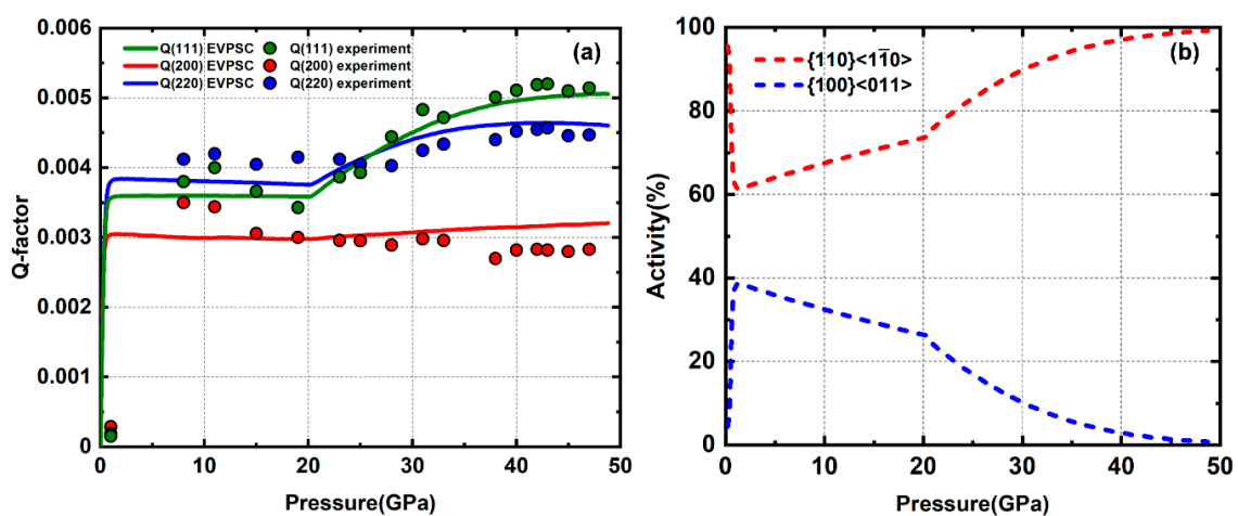
Figure 4. (a) Experiment and modeled Q-factors of pure MgO; (b) slip system activity; replotted from [48].
