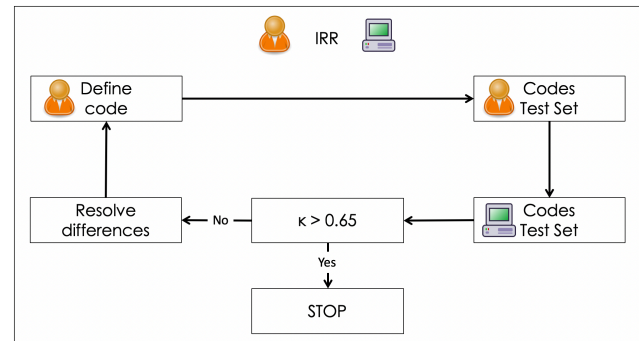
Figure 1: Workflow for establishing inter rater reliability using the Common Method (shown here with kappa).
