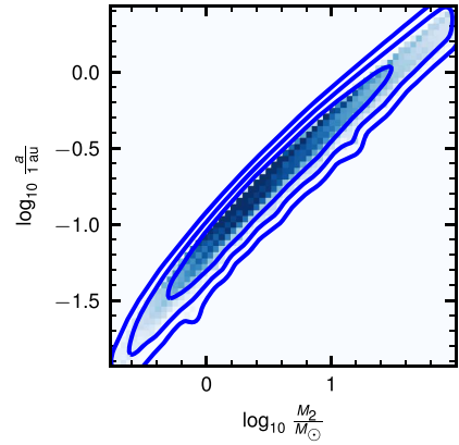
Figure 9. The distribution of semimajor axis of the binary system and mass of a secondary that could have produced S5-HVS1 via the Hills mechanism. The contours encircle the 68 per cent, 95 per cent, and 99.7 per cent posterior volumes.
