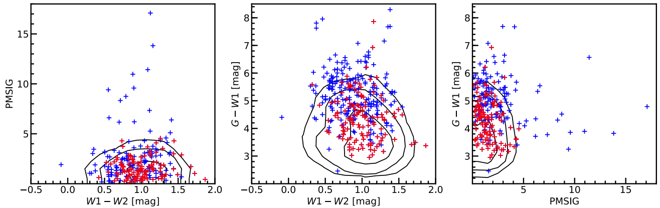
Figure 10. Distributions of the top three most important features, W1 - W2 , PMSIG , and G - W1 , for the 333 known lensed quasar images in the Gaia –unWISE sample. The black contours correspond to distributions of AGNs in the training set. Compared to AGNs in the training set or lensed quasar images recovered in the C75 catalogue (red symbols), lensed quasar images that are not in the C75 catalogue (blue symbols) tend to have smaller W1 - W2 and larger PMSIG and G - W1 .
