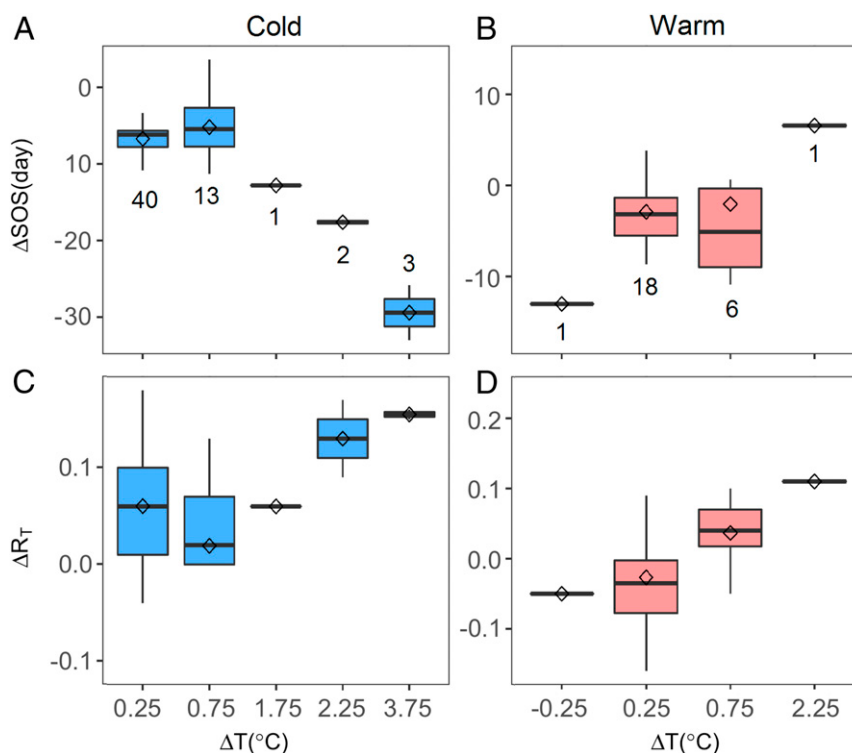
Fig. 3. Changes in (A and B) \Delta SOS and (C and D) \Delta R_T with \Delta T in cold and warm regions. \Delta SOS = SOS_{Urban} - SOS_{Rural} , \Delta R_T = R_{TUrban} - R_{TRural} , and \Delta T = T_{Urban} - T_{Rural} . Negative \Delta SOS represents an earlier urban SOS, and positive \Delta R_T represents a decreased magnitude in SOS response to temperature in urban areas. Positive \Delta T represents UHI effect. Results are shown at 0.5 °C bin of \Delta T . The x axis is the mean \Delta T in each bin. The central line and the rhombus represent the median and mean values, respectively. The lower and upper hinges correspond to the 25th and 75th percentiles, respectively. A and C are the results for cold regions (blue), and B and D are the results for warm regions (red). Sample sizes are indicated using numbers for each bin (shown in A and B).
